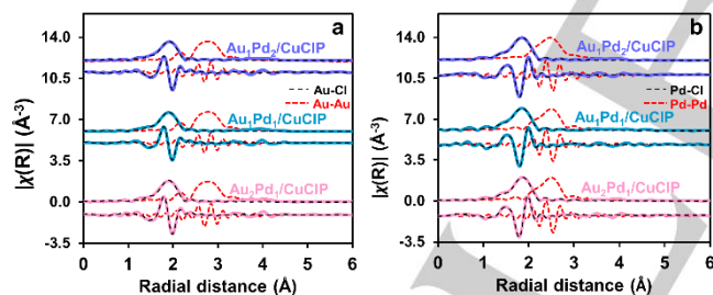
Figure 5. The magnitude and real component of the k^2 weighted Fourier transform of the EXAFS for the (a) Au edge and (b) Pd edge of \text{Au}_x\text{Pd}_y/\text{CuClIP} catalysts. Fitting parameters are provided in Table S2.
