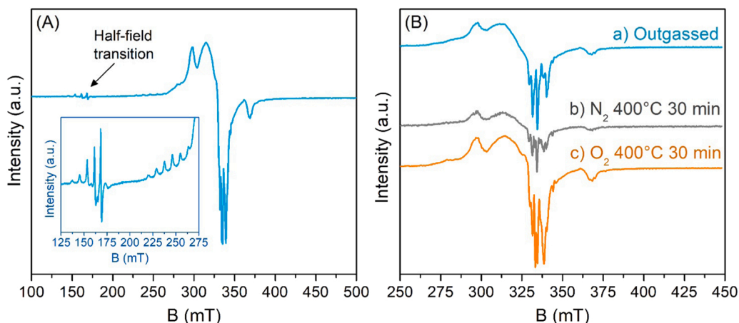
Fig. 2. Complete EPR spectrum of the Ce95Cu5 sample acquired at -196\text{ }^{\circ}\text{C} after outgassing the powder (A); in the inset, the half-field transition region is magnified. EPR spectra collected at -196\text{ }^{\circ}\text{C} after treating the Ce95Cu5 catalyst in different ways (B): after outgassing the sample (a), after thermal treatment in \text{N}_2 at 400\text{ }^{\circ}\text{C} for 30 min (b), and after thermal treatment in \text{O}_2 at 400\text{ }^{\circ}\text{C} for 30 min (c).
