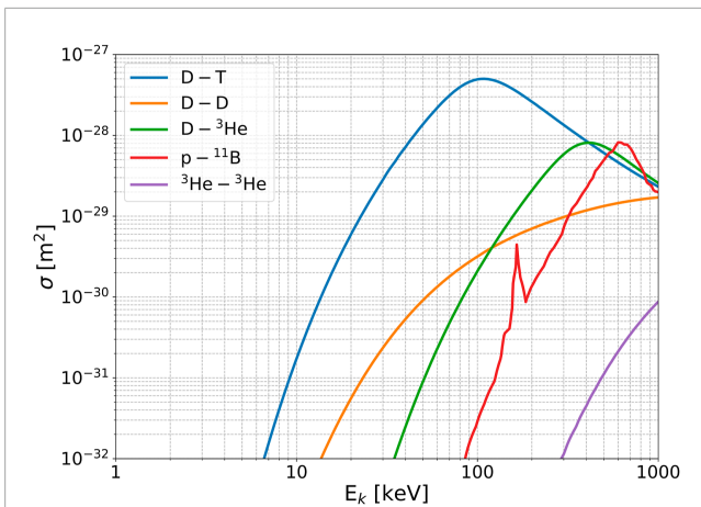
FIGURE 2 Experimental cross sections ( \sigma ) for the most relevant fusion reactions. Most of the projects are based on D-T reactions, which show the highest cross section at low energy. The x-axis shows the energy in the laboratory frame. Libraries: ENDF/B-VIII.0 (D-D, D-T, D- ^3\text{He} , ^3\text{He} - ^3\text{He} ) (Brown et al., 2018) and EXFOR (p- ^{11}\text{B} ) (Otuka et al., 2014). The (p- ^{11}\text{B} ) cross section is the result of the interpolation of the experimental data in the EXFOR library.
