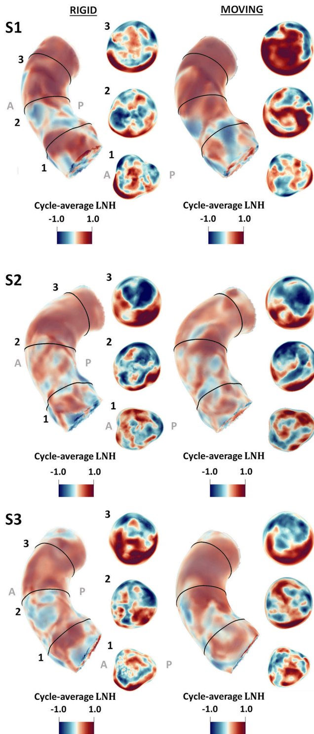
Fig. 7. Impact of aortic motion on helical flow topological features in the AAO: volume maps of cycle-average LNH in the rigid- and moving-wall models. Positive (red) and negative (blue) LNH values indicate counter-rotating flow structures. (For interpretation of the references to color in this figure legend, the reader is referred to the web version of this article.)
