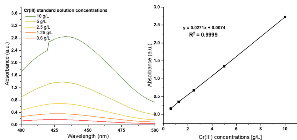
Figure 10. UV-Vis spectra of chromium (III) chloride hexahydrate standard solutions with a similar concentration of real samples, RT, and neutral pH, with the associated calibration curve ( \lambda_{\text{MAX}} = 423 nm).
