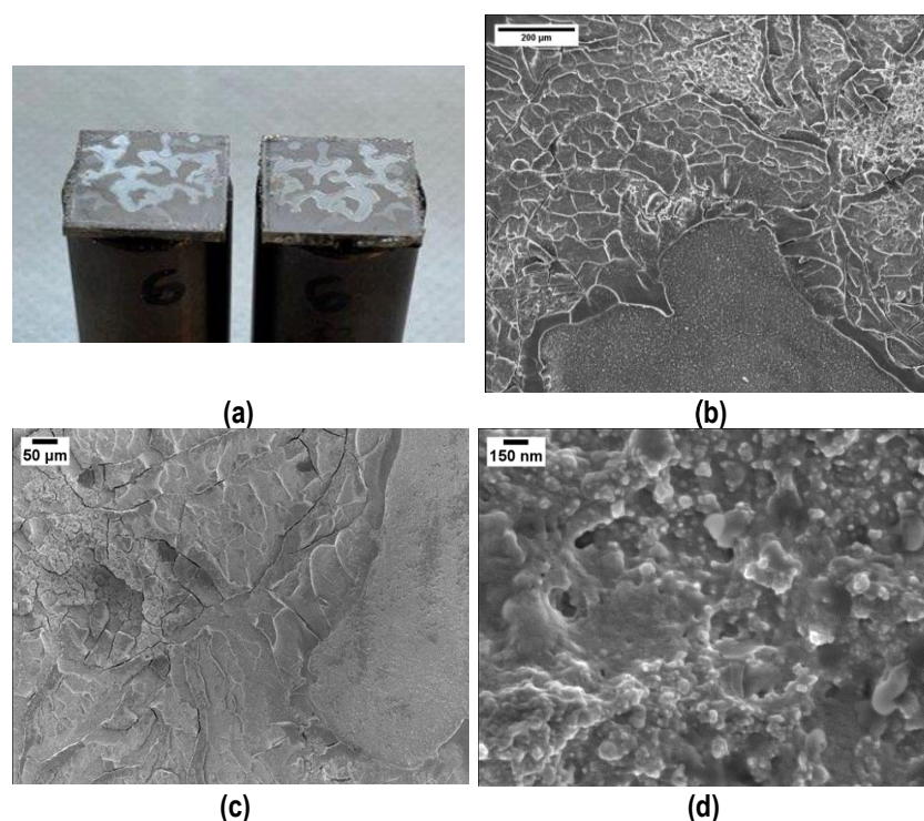
Figure 12. Typical cohesive fracture surface after tensile test on samples joined using polymer loaded with 48 wt% silica nanoparticles: visual appearance (a) and FESEM (b–d) of the joining material.
