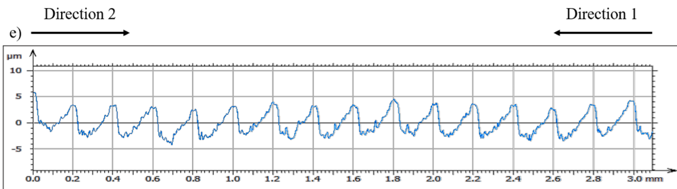
Fig. 1. SEM micrographs of the Laser Textured Al CC at magnifications of a) 5kX and b) 30 kX. Optical profilometry 3D images of the surface of the c) pristine Al CC and d) Laser Textured Al CC. e) Contact profilometry line scan of the asymmetric grooves obtained on the Laser Textured Al CC. The direction 1 and 2 (arrows) are related to the adhesion measurements described in Section 3.2.
