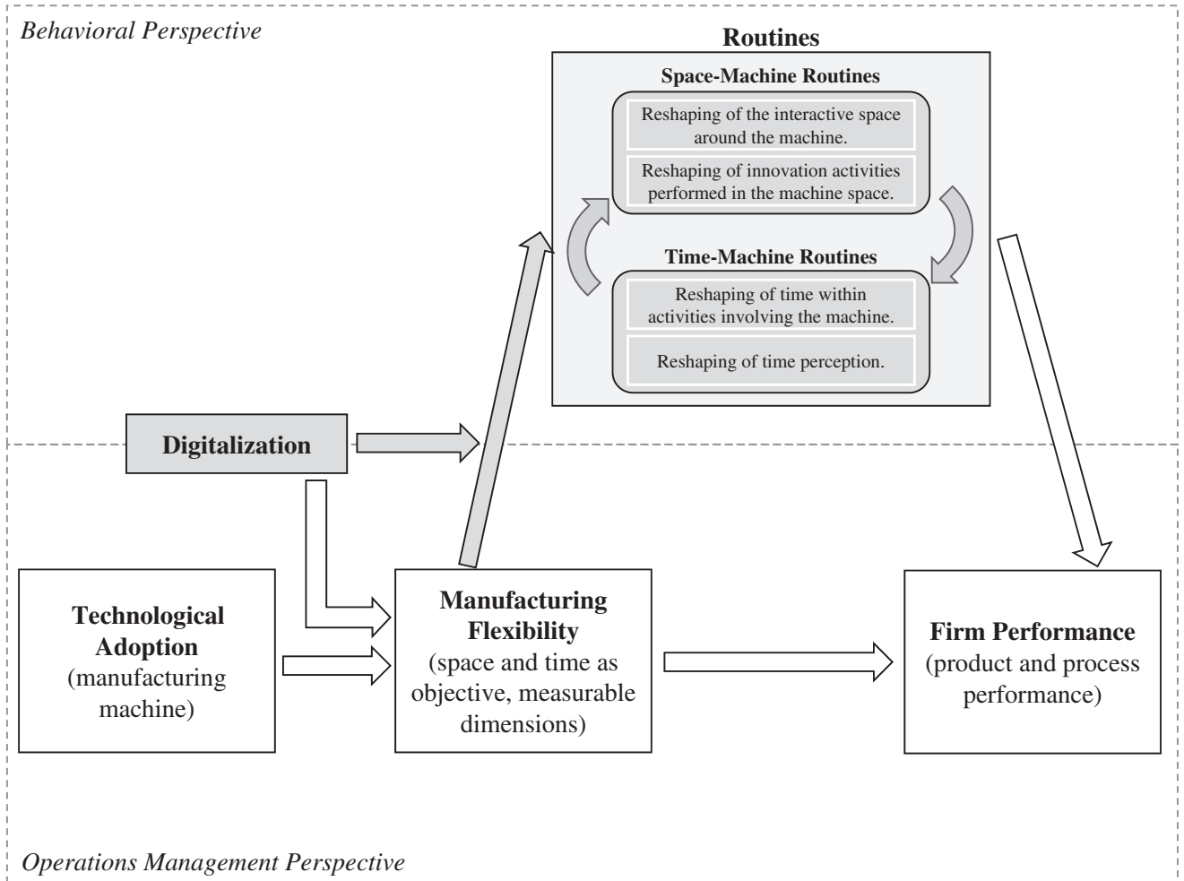
Figure 2. Conceptual Framework: Manufacturing Flexibility, Digitalization, and Routines. Note: White shapes: elements from the literature review. Gray shapes: elements developed in this study
