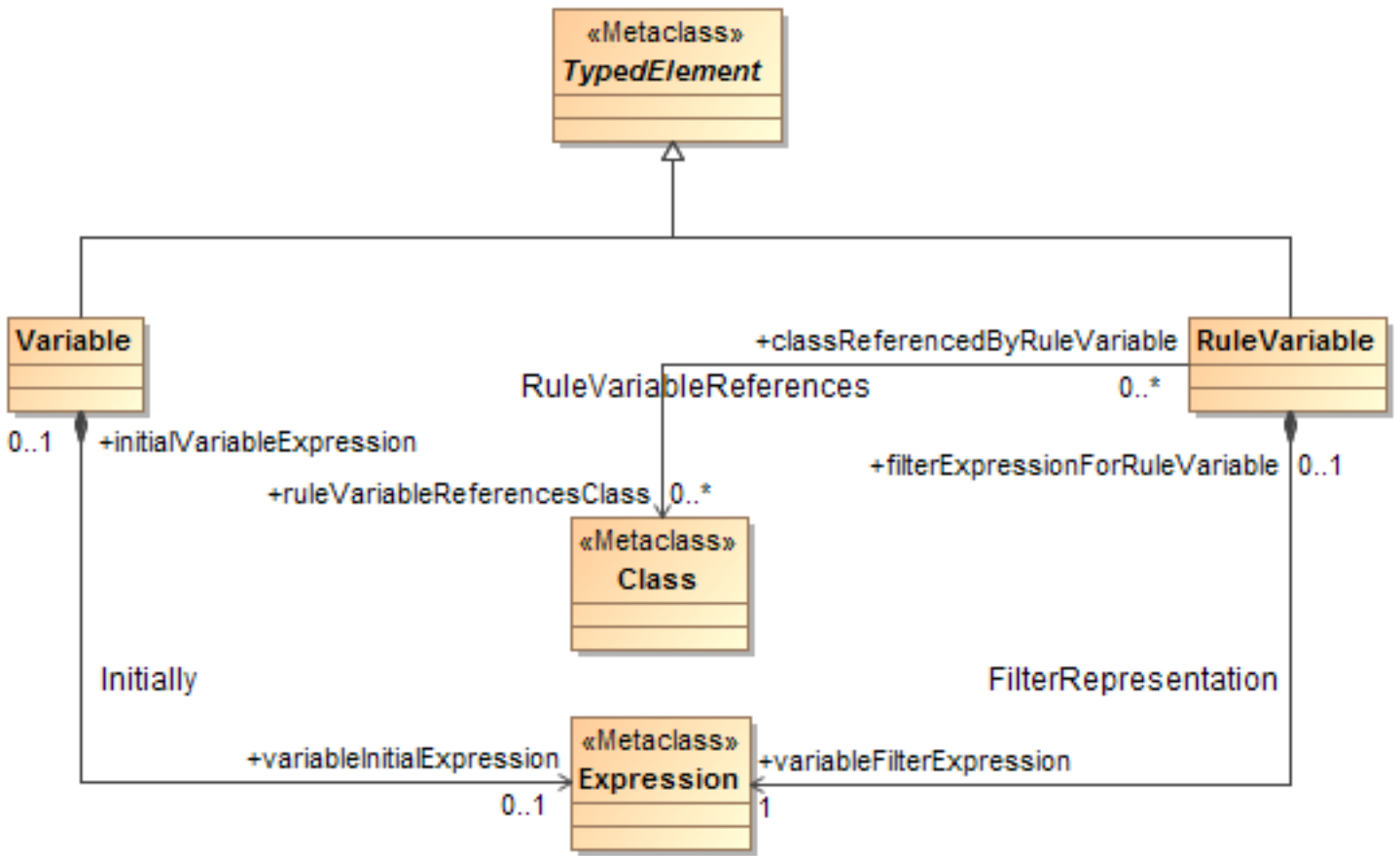
Figure 7.4 - PRR RuleVariable Classes
