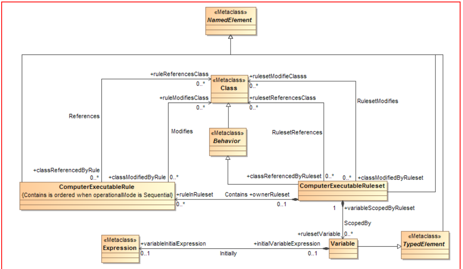
Figure 7.1 - PRR Concept Classes
