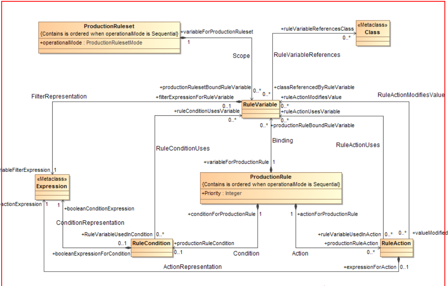
Figure 7.3 - PRR ProductionRule Classes
