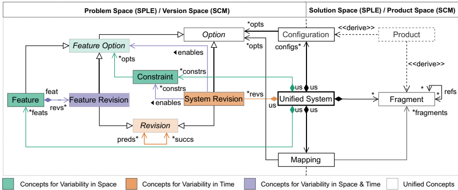
Fig. 4 UML class diagram of the conceptual model for unifying concepts for variability in space and time
