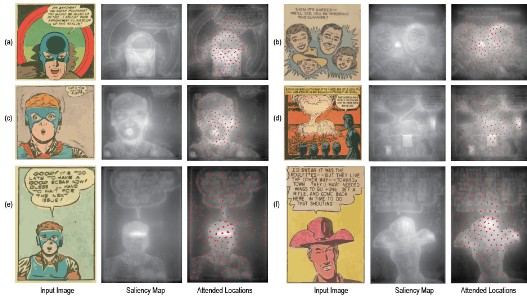
Fig. 10. Computation of saliency-based visually attended locations using Judd et al.'s saliency model coupled with Winner-Take-All network on six comic panels. In each comic panel (left) Original input image, (middle) Saliency map generated using Judd et al.'s saliency model, (right) Visually attended locations marked in red points have been overlaid on saliency maps.
