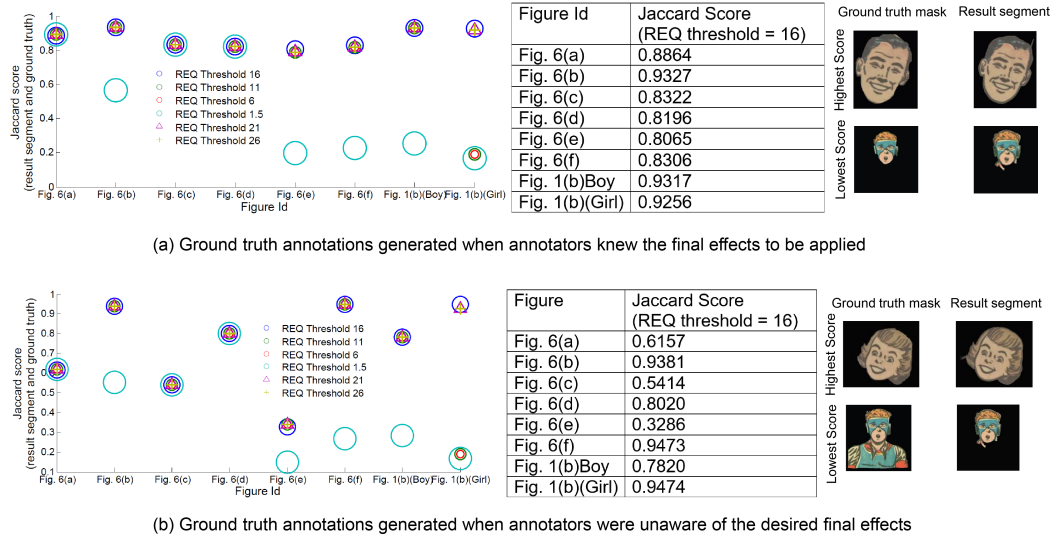
Fig. 7. Quantitative evaluation of segmentation results. The ground truth masks and our results for the segments with the highest and lowest Jaccard scores are also shown here.
