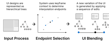
Figure 6: An overview of FrameKit's computational approach to UI adaptation. Keyframes contain UI designs that are represented as trees, associated with context variables. The system finds relevant keyframes (endpoints) based on a target query. An edit sequence is computed from the endpoints which is used to generate additional variations.
