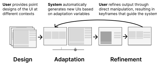
Figure 5: FrameKit's overall workflow. Design phase: authors specify point designs of the UI associated with adaptation parameters. Adapt phase: tool generates additional variations of a UI for unseen contexts. Refine phase: user refines the generated output or provide additional keyframes to guide algorithm behavior.
