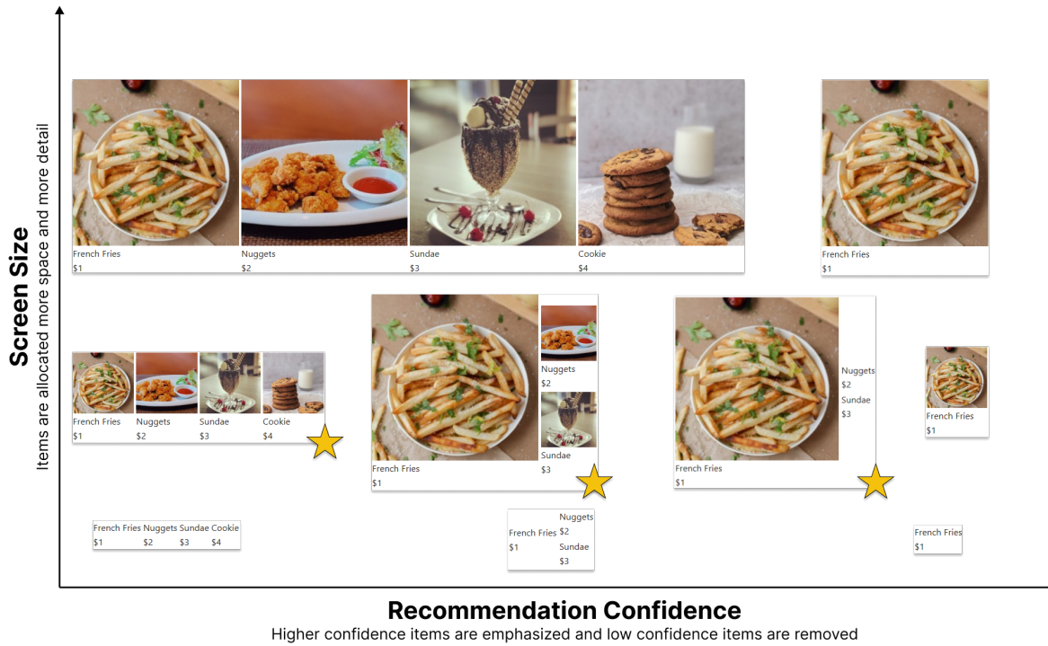
Figure 4: The adaptivity of the Food Menu app represented in a 2-D space. There are two adaptation parameters, i ) screen size and ii ) recommendation confidence, and we show 9 adaptations of the app in this space, although there are more generated variations that are not shown due to space constraints. As screen size is increased, items are allocated more space and detail. As recommendation confidence is increased, higher confidence items are emphasized through relative size while low confidence items are removed. In this example, the UI variations with a star icon were automatically generated as frames, but the user made small edits, turning them into keyframes. A video is provided in the supplemental material to show the originally generated frames and user edits.
