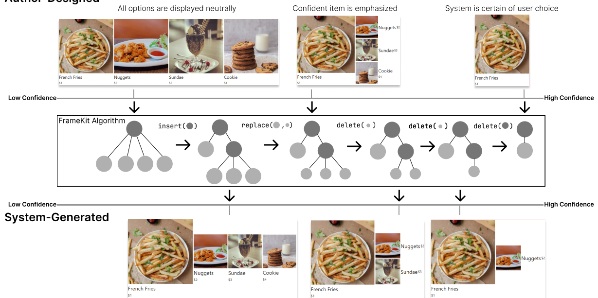
Figure 1: FrameKit is a tool for authoring adaptive user interfaces based on a ‘keyframe’ metaphor. In the example above, an author designs an interface for a recommendation system that adapts the size of UI elements based on the system’s confidence in a recommendation. The author provides three ‘keyframe’ designs for how the UI should look at different confidence values (top). The system applies a computational approach (middle) to generate additional variations by interpolating between the keyframes (bottom).
