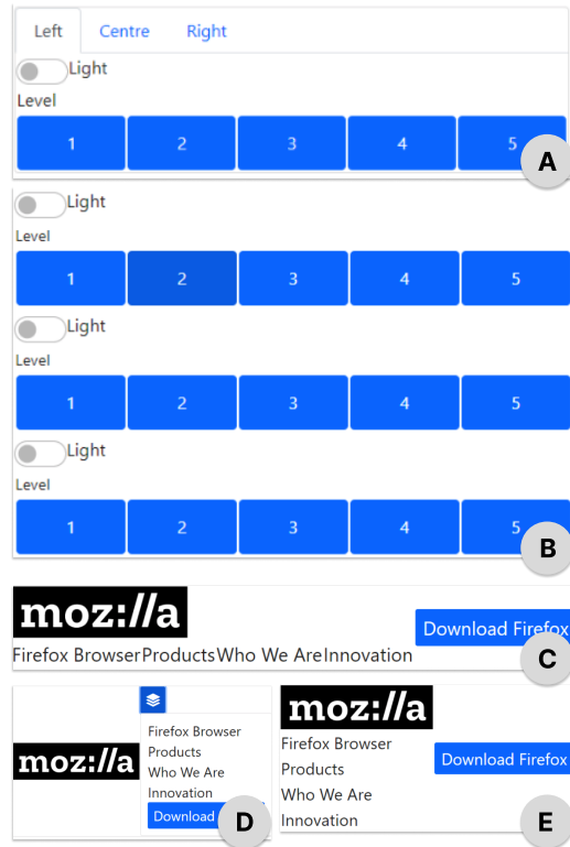
Figure 9: Examples of keyframes from our user study. A) is a manually created SUPPLE keyframe (P10). B) is an automatically generated SUPPLE keyframe (P10). C) and D) are manually created Mozilla keyframes (P9). E) is an automatically generated Mozilla keyframe (P9).
