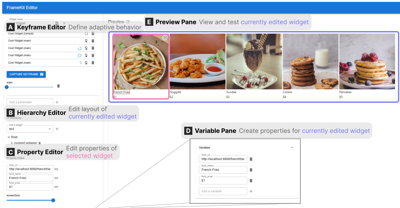
Figure 2: FrameKit’s authoring interface is divided into several regions. The Hierarchy and Property Editors (B & C) are used to create variations of the UI, which are associated with different parameters in the Keyframe Editor (A). The Preview Pane (E) is used to test the AUI. The Variable Pane (D) exposes editable values for use when nesting the current widget within other widgets.
