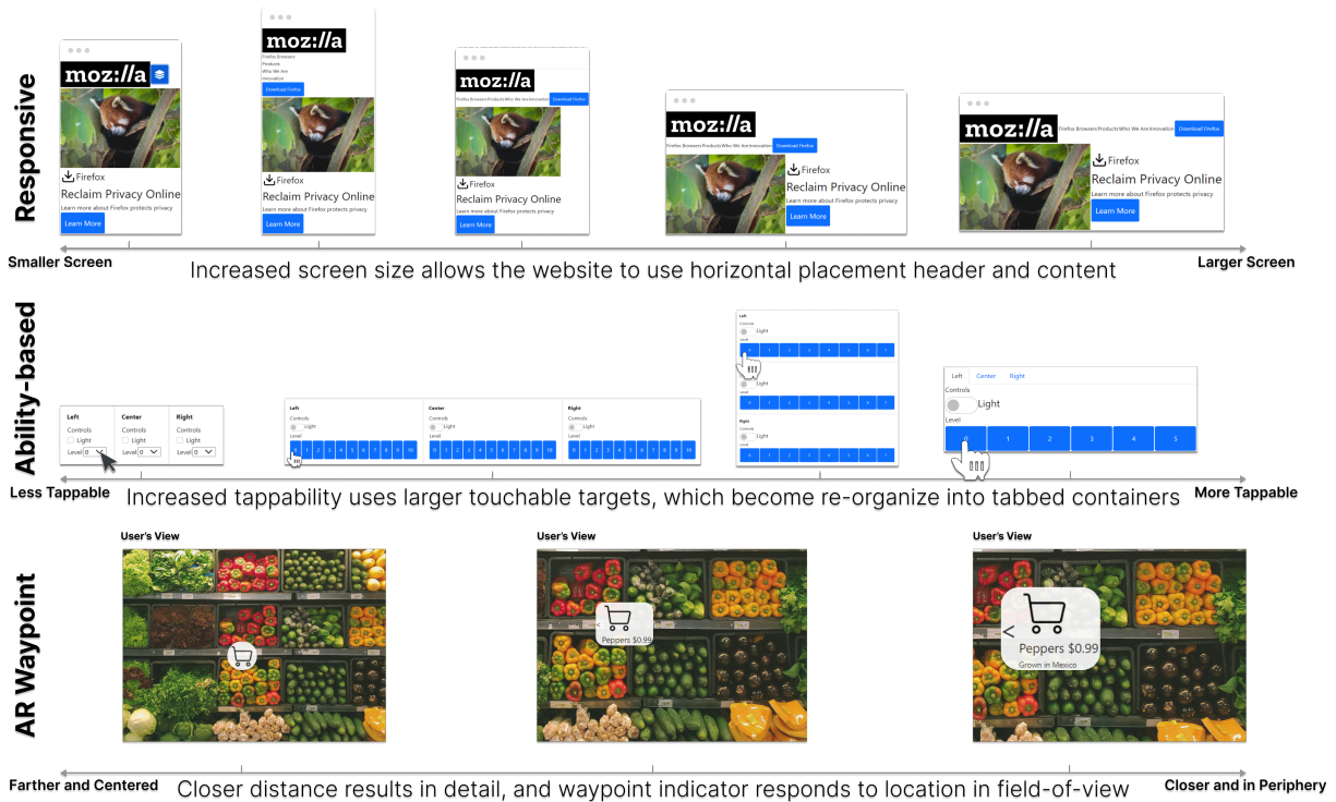
Figure 7: The Responsive (Top), Ability-based (Center), and AR Waypoint (Bottom) examples are represented along their adaptation parameters. The Responsive UI adapts to larger screen sizes by expanding the header menu and re-positioning the page content. The Ability-based UI is based on an example use-case of SUPPLE [26], where controls are made easier to tap while maintaining the same window size through container changes. The AR Waypoint is an example of a UI that shows more information at closer distances while also using directional indicators that adapt to the item’s location in the user’s field of view. The second frame of the Responsive UI, the second and third frames of the Ability-based UI, and the second frame of the AR Waypoint are automatically generated from the user-edited keyframes.
