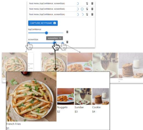
Figure 3: FrameKit automatically generates variations of the UI based on keyframes associated with adaptation parameters. This figure shows the variations of a widget from the food menu UI that was generated from manually provided keyframes (the endpoints) which depend on two parameters.
