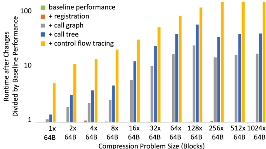
Fig. 9 Analysis of RSMT Performance Overhead
