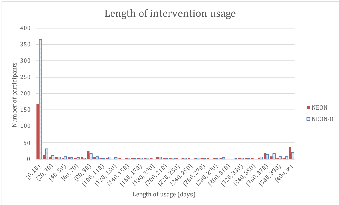
Figure S1 - Length of time between first and last narrative request, for both NEON and NEON-O participants.
