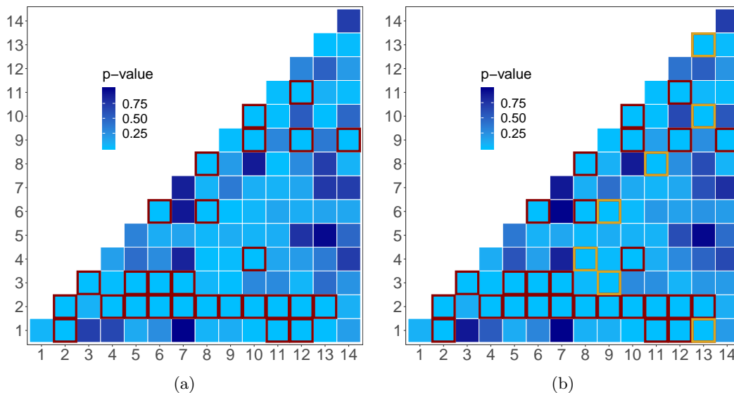
Figure 3: Results of the cell-level significance tests of the unweighted (left) and weighted (right) network averages. Each tile corresponds to a cell, with tiles colored according to p-values. The cells highlighted by red or yellow squares indicate those for which one or both of the weighted and the unweighted procedures rejected the null hypothesis. Cells highlighted in red are those that were rejected by both the unweighted and weighted tests after Benjamini-Hochberg correction at false discovery rate 0.01. Cells highlighted in yellow in the weighted plot (right) correspond to those rejected by the weighted procedure, but not its unweighted counterpart. All cells rejected by the unweighted procedure were also rejected by the weighted procedure. Numbering of the axes corresponds to the brain region numbering given in Table 1
