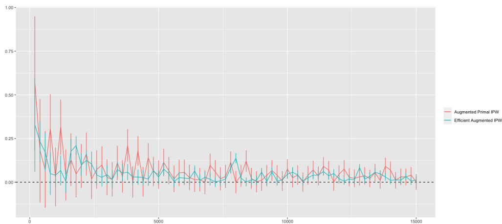
Figure 9: Comparing bias and variance behavior of the Augmented Primal IPW and efficient AIPW as a function of sample size, using the ADMG in Fig. 3. The error bars illustrate the variance of the corresponding influence function.
