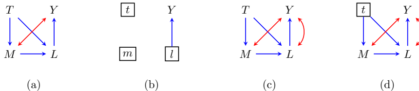
Figure 1: (a) Example of an ADMG where the missing edge between T and Y corresponds to a Verma constraint; (b) CADMG corresponding to the kernel q_Y(T | L) that shows the Verma constraint in (a); (c) Example of an ADMG where the missing edge between T and Y does not correspond to any equality constraint; (d) The CADMG \phi_{-\{Y\}}(\mathcal{G}) when checking for equality constraints in (c).
