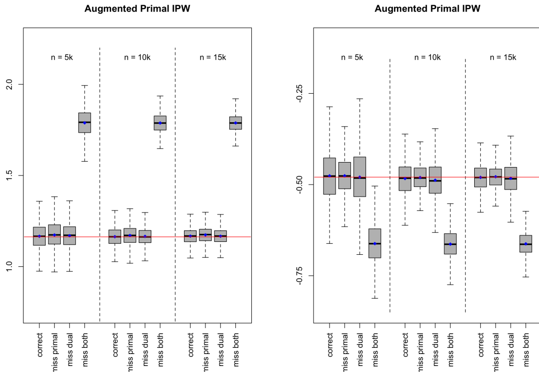
Figure 8: Demonstrating the double robustness of the Augmented Primal IPW estimator. The boxplot panel on the (left) uses the ADMG in Fig. 2(b), and the one on the (right) uses the ADMG in Fig. 3. The red dashed lines indicate the true values of the ACE.
