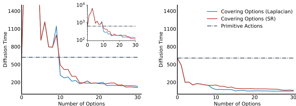
Figure 30: Average (left) and median (right) diffusion time in the four-room domain induced by covering options when computed with the SR and the eigenvectors of the graph Laplacian, in closed-form. The inset plot on the left figure depicts, in log-scale, the range the diffusion time lies.
