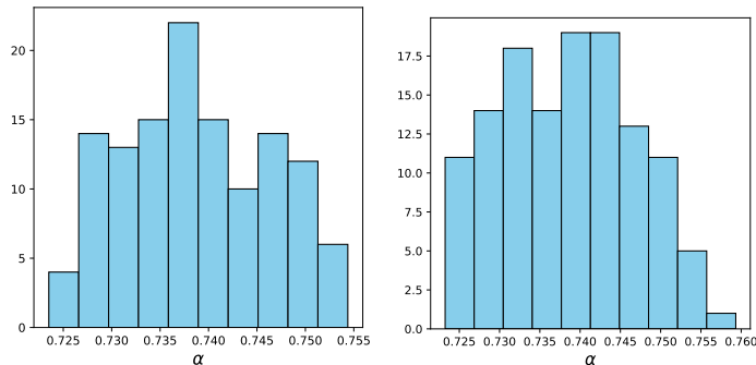
Figure 8: Inferred \alpha values for gen. BFRY on MNIST (left) and Fashion MNIST (right).
