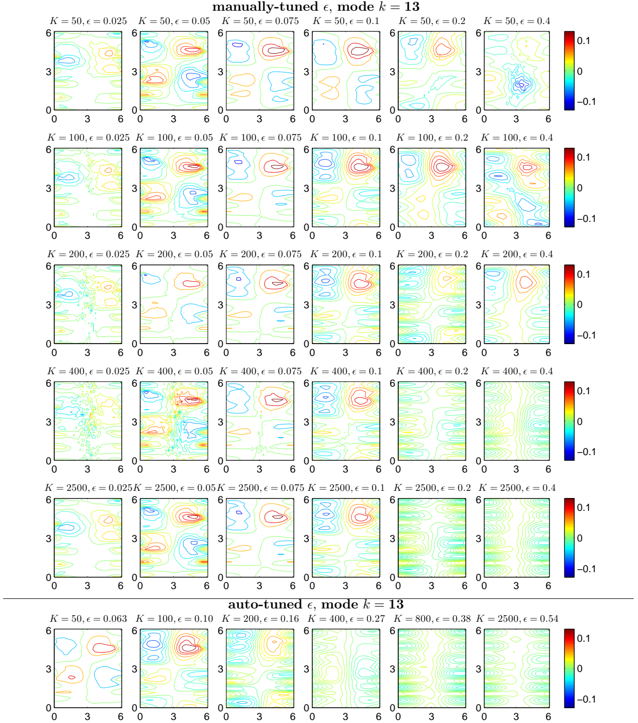
Figure 16: 2D general torus in \mathbb{R}^{21} . Mode k = 13 . Comparison of eigenfunctions of Laplace -Beltrami among various DMs with different K -nearest neighbors and bandwidth \epsilon . Panels from the first row to the fifth row correspond to manually-tuned \epsilon for K = 50, 100, 200, 400, 2500 , respectively. Panels in the last row correspond to auto-tuned \epsilon for various K . The randomly distributed N = 2500 data points on the manifold are used for computing the eigenvalue problem.
