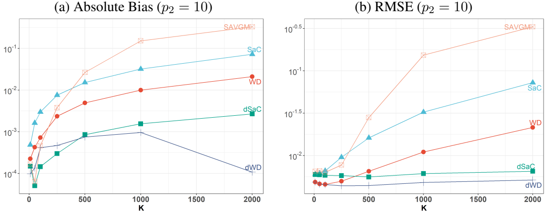
Figure 1: Average simulated bias (a) and the root mean squared errors (RMSE) (b) of the weighted distributed (WD) (red circle), the split-and-conquer(SaC) (blue triangle), the debiased split-and-conquer (dSaC) (green square), the debiased weighted distributed (dWD) (purple cross), the sub-sampled average mixture SAVGM (pink square cross) estimators, with respect to the number of data block K for the logistic regression model with the dimension p_2 of the nuisance parameter \lambda_k being 10, and the full sample size N = 2 \times 10^6 .
