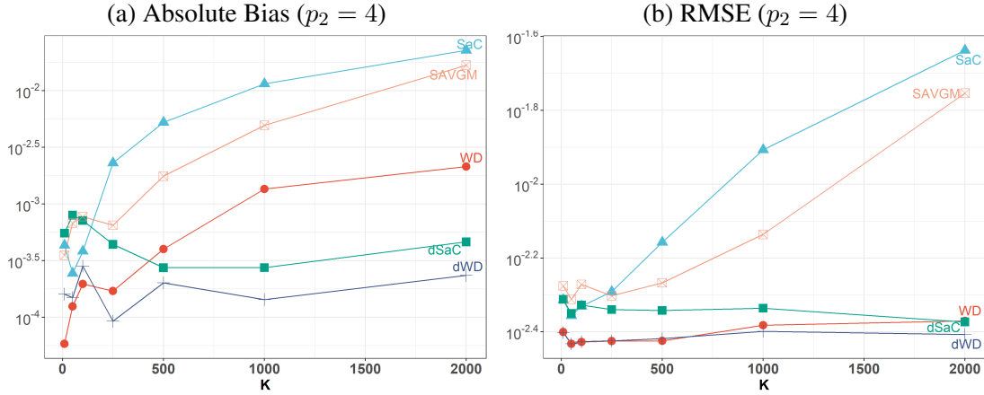
Figure 3: Average simulated bias (a) and the root mean squared errors (RMSE) (b) of the weighted distributed (WD) (red circle), the split-and-conquer(SaC) (blue triangle), the debiased split-and-conquer (dSaC) (green square), the debiased weighted distributed (dWD) (purple cross), the sub-sampled average mixture SAVGM (pink square cross) estimators, with respect to the number of data block K for the logistic regression model with the dimension p_2 of the nuisance parameter \lambda_k being 4, and the full sample size N = 2 \times 10^6 .
