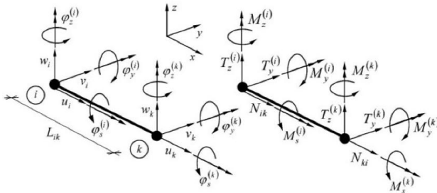
Fig. 3. Two-node spatial bar finite element
