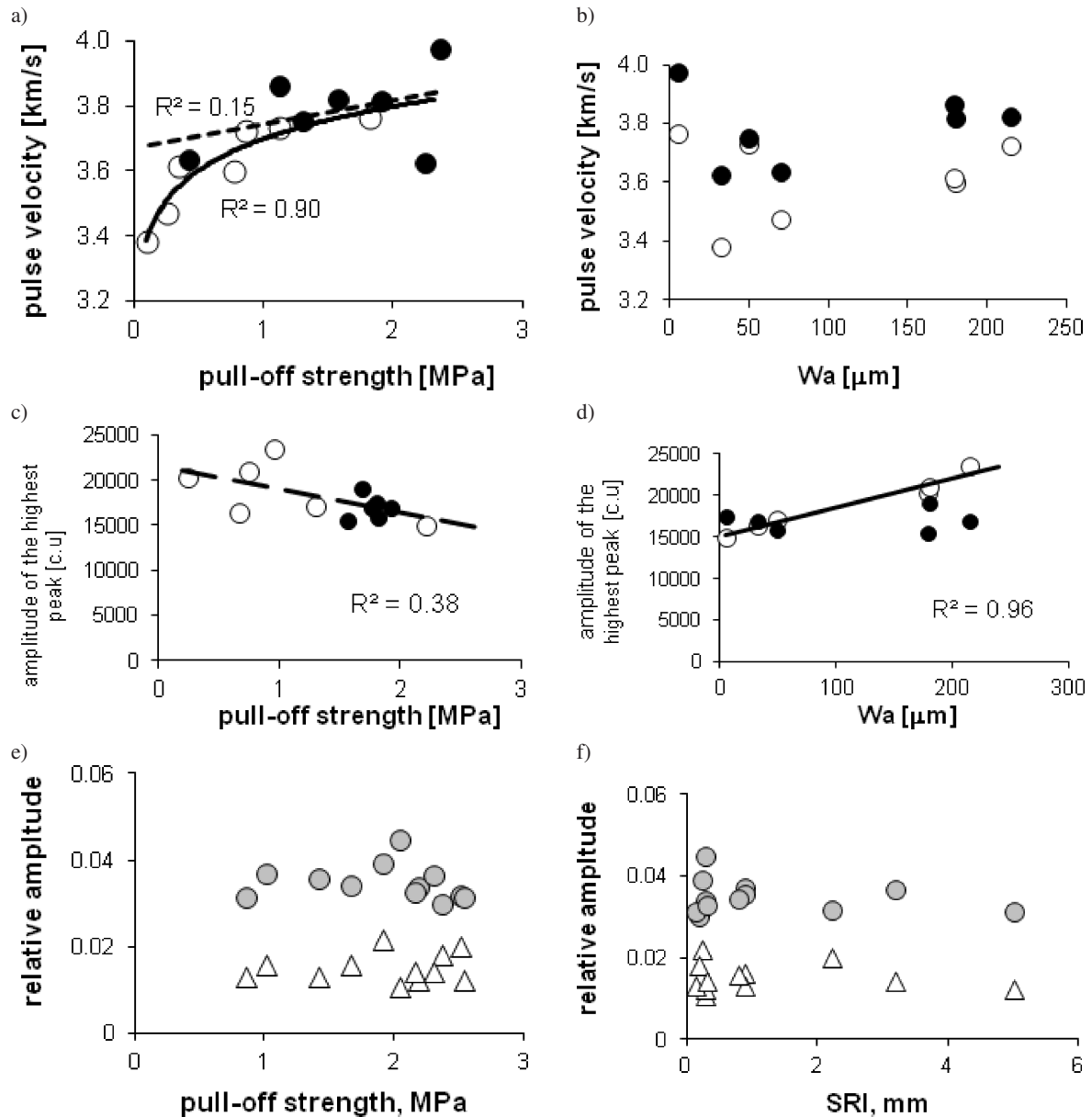
Fig. 4. Relationships between parameters describing stress wave propagation and parameters describing repair system quality: a) pulse velocity vs. pull-off strength, b) mean waviness of profile, W_a , vs. pulse velocity, c) amplitude of the highest peak of frequency spectrum of ultrasonic signal (c.u. – conventional unit) vs. pull-off strength, d) amplitude of the highest peak of frequency spectrum of ultrasonic signal vs. mean waviness of profile, W_a ; (concrete substrate C20/25, overlays with (●) and without (○) the bond coat; adopted from Ref. 20. Amplitude of bottom (●) and interface (Δ) frequency peaks versus: e) pull-off strength, f) surface roughness index, SRI (adopted from Ref. 32)
