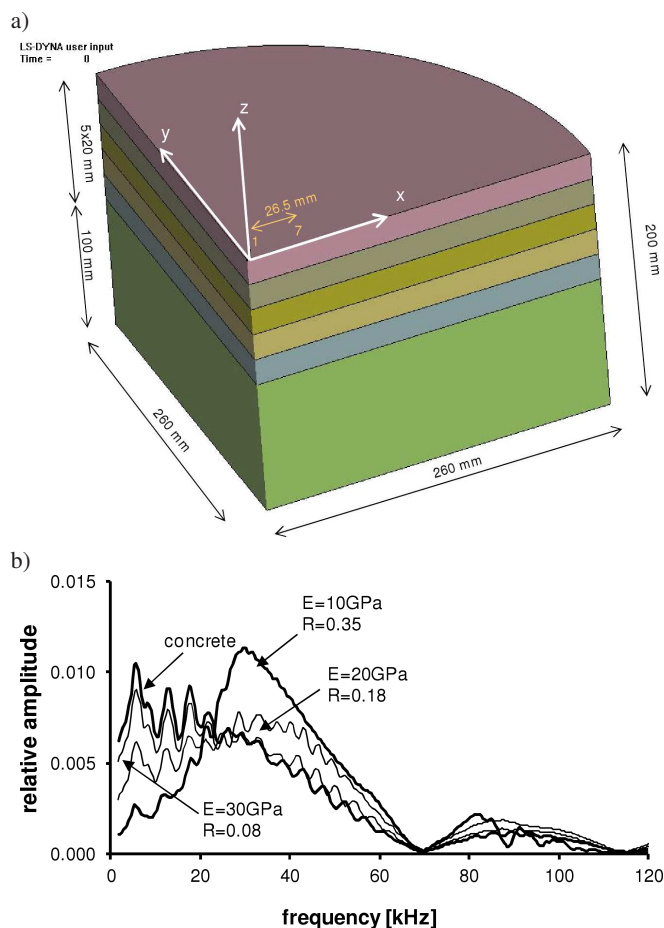
Fig. 2. a) FEM model of repair system and b) frequency spectra for repair materials with different reflection coefficient R (details in the text); adopted from Ref. 17
