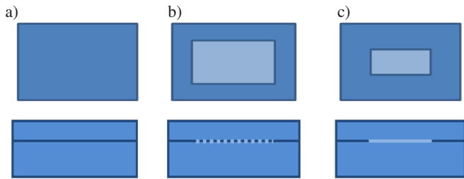
Fig. 6. Different types of defects at interface: a) no defect – reference slab, b) demoulding oil (55×35cm), c) rectangular plastic sheet (40×20 cm); in each case: concrete slab dimensions of 60×80×8 cm and repair material thicknesses of 5 or 8 cm
