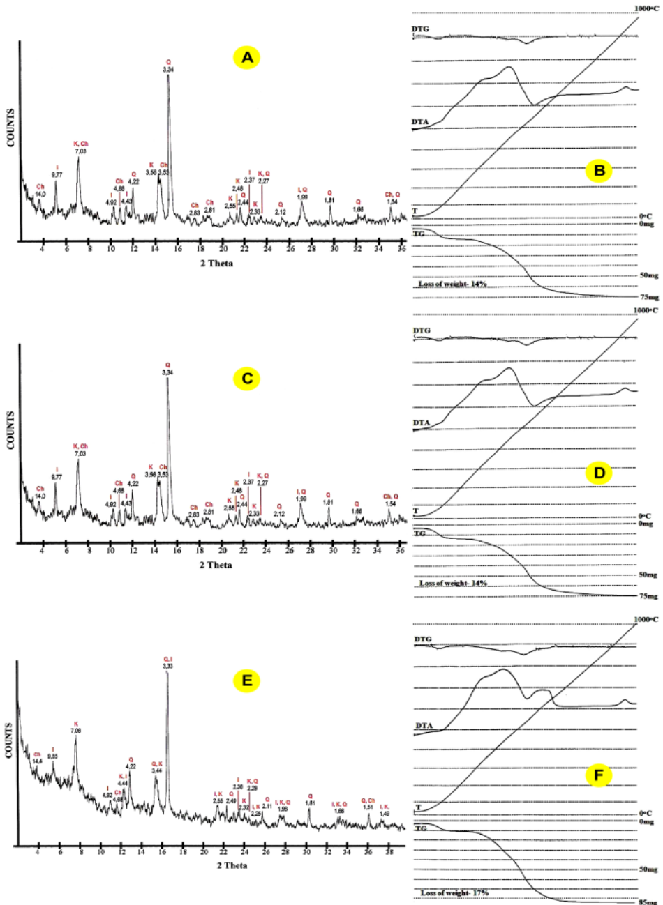
Plate 10. X-ray diffraction patterns and derivathograms of claystones (samples 5, 7, 11).
