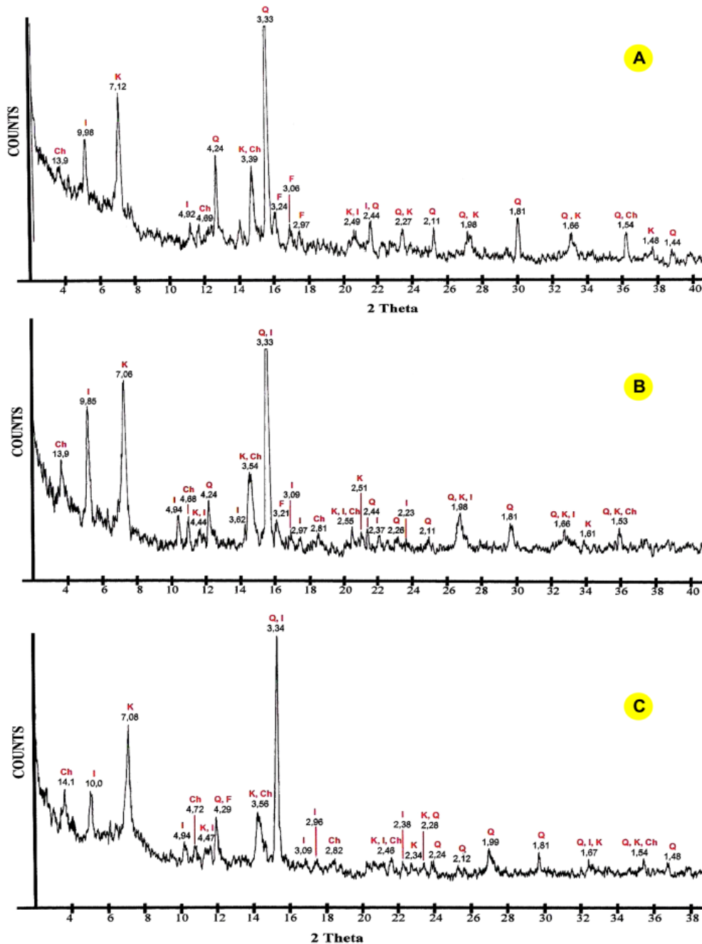
Plate 8. X-ray diffraction patterns of mudstones.
