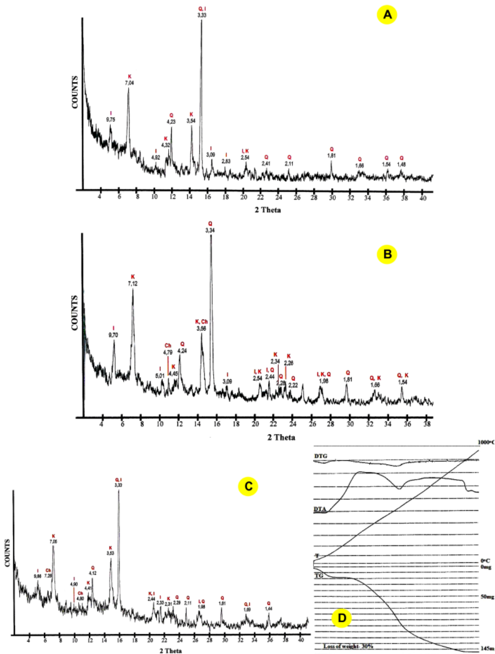
Plate 9. X-ray diffraction patterns of samples 12, 14 (mudstones) and 1 (claystone) and derivathogram of sample 1.
