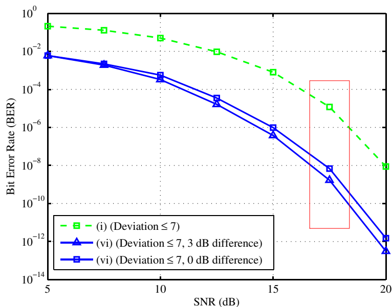
Figure 12 BER under BRAN-A channel.
