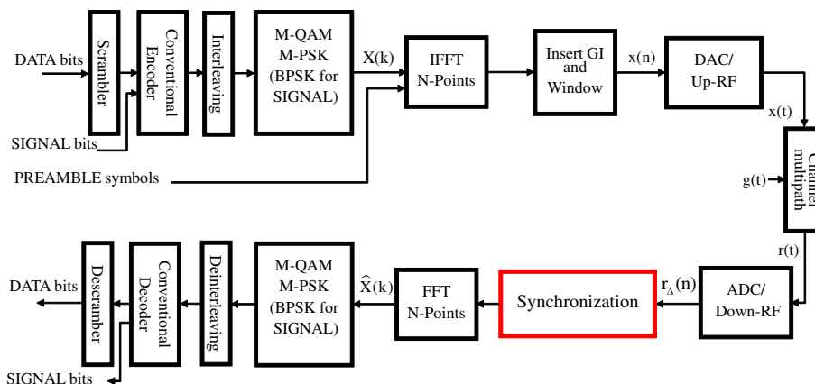
Figure 2 Wireless communication system using OFDM.
