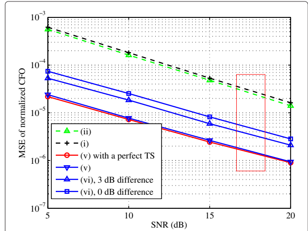
Figure 6 MSE of normalized CFO under BRAN-A channel.
