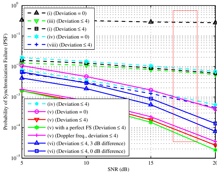
Figure 9 PSF under COST207-RA channel.
