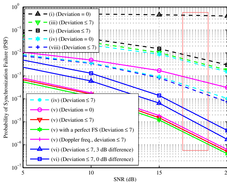
Figure 10 PSF under BRAN-A channel.
