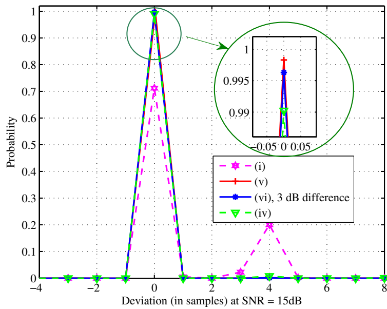
Figure 7 Deviation with respect to the true time position of a physical packet under COST207-RA channel.
