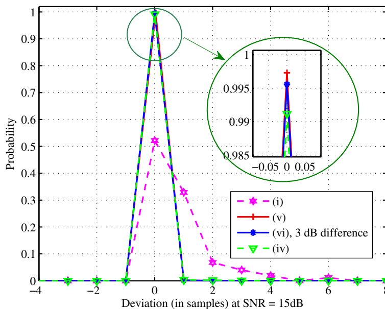
Figure 8 Deviation with respect to the true time position of a physical packet under BRAN-A channel.
