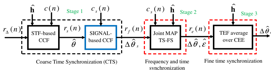
Figure 3 Proposed time and frequency synchronization algorithm.
