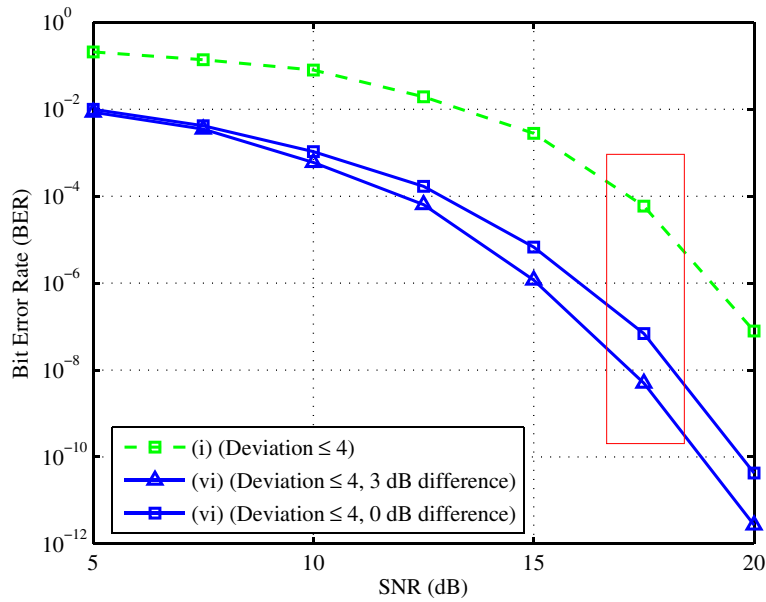
Figure 11 BER under COST207-RA channel.
