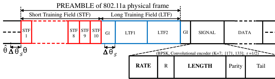
Figure 1 IEEE 802.11a physical packet.
