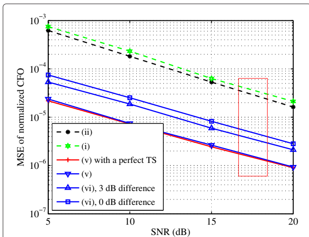
Figure 5 MSE of normalized CFO under COST207-RA channel model. The rectangular box represents the operating area of the 802.11a standard.
