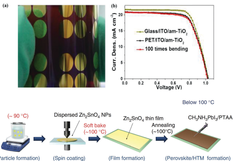
Fig. 2 Above: (a) Photograph of one of the best performing flexible PSC (PET/ITO/TiO 2 /CH 3 NH 3 PbI 3-x Cl x /spiro-OMeTAD/Au) reported at the time of publication with sputtered TiO 2 compact layer; (b) JV scan of the best devices on both glass and PET, showing also the curves after bending the latter for 100 times (radius of curvature not given). 99 Reproduced from ref. 99 with permission from The Royal Society of Chemistry. Below: Scheme of the low temperature synthesis and application of Zn 2 SnO 4 nanoparticles for fabricating flexible PET/ITO/Zn 2 SnO 4 /CH 3 NH 3 PbI 3 /PTAA/Au cells. 55 Adapted from High-performance flexible perovskite solar cells exploiting Zn 2 SnO 4 prepared in solution below 100 °C, Nat. Commun. , 6 , 55 Copyright © 2015, Rights Managed by Nature Publishing Group.
