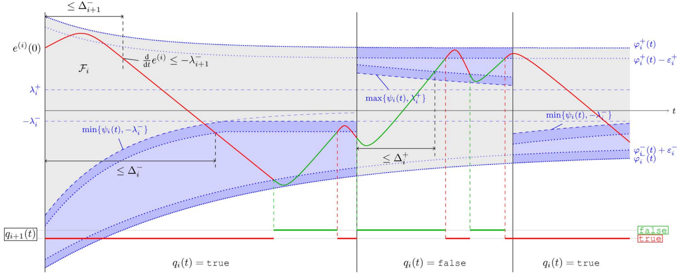
Fig. 6. Illustration for understanding the feasibility property of the switching logic \mathcal{S}_i together with (q_i, \psi_i) in the intermediate closed loop as shown in Fig. 5. Condition (17a) ensures that e^{(i)} remains within the funnel \mathcal{F}_i (provided the initial value e^{(i)}(t_0) was safely contained in \mathcal{F}_i ), conditions (17b) and (17c) ensure that e^{(i)} remains within the blue shaded regions as long as initially e^{(i)}(t_0) was safely contained in the corresponding region; finally, conditions (17d) and (17e) ensure that within a time span of length at most \Delta_i^\pm the signal e^{(i)} reaches the blue shaded region. Additionally, the output q_{i+1} of the block \mathcal{B}_i is indicated.
