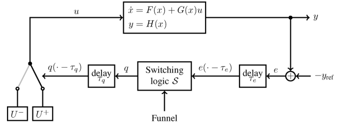
Fig. 7. Closed loop with additional time delays \tau_e for the error signal e and \tau_q for the switching signal q .
