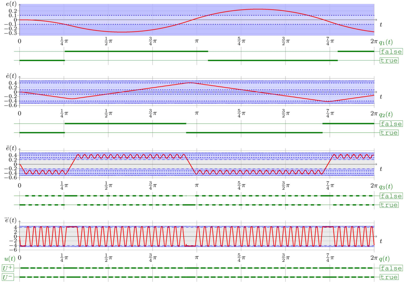
Fig. 9. The error and its derivatives — with corresponding switching variables —. The funnel boundaries are drawn as ..... (note that the funnel boundaries \varphi_0^{\pm} \equiv 1 are not in the picture), the safety distances are shown as .....
