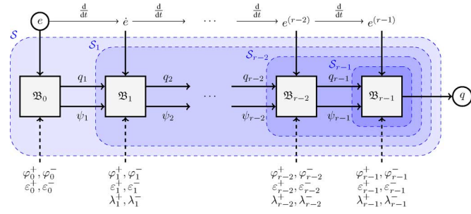
Fig. 2. Illustration of the structure of the switching logic (9). The meaning of the meta blocks S_1, \dots, S_{r-1} will be discussed in Section VI, in particular, S_i is given by (16).
