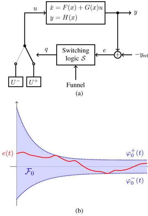
Fig. 1. Overall setup for the bang-bang funnel controller. (a) Overall system structure. (b) The funnel \mathcal{F}_0 : A time-varying error bound.
