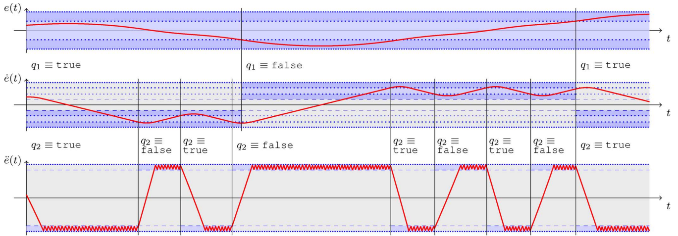
Fig. 4. Schematic illustration of the closed-loop behavior of the bang-bang funnel controller for relative degree three case and constant funnel boundaries ; the desired increase rate \lambda_1^+ = \lambda_1^- > 0 and \lambda_2^+ = \lambda_2^- > 0 are drawn with \cdot , the desired regions for e^{(i)} in \mathcal{F}_i are highlighted as well as the safety region (given by \varepsilon_0^+ = \varepsilon_0^- > 0 and \varepsilon_1^+ = \varepsilon_1^- > 0 drawn with \cdot ; \varepsilon_2^\pm > 0 is so small that it is not shown).
