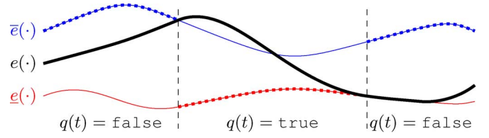
Fig. 3. Illustration of the basic switching predicate \mathfrak{S} and the corresponding DLS (11) for some given “input signal” e(\cdot) (thick solid line). The dots indicate which switch trigger is active. Note that it is not assumed that e(\cdot) is always contained within the lower switching trigger \underline{e}(\cdot) and the upper switch trigger \bar{e}(\cdot) and it is possible that e(\cdot) is identical with one of the switching triggers for some time.
