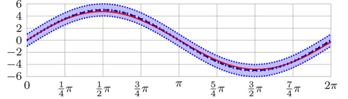
Fig. 8. Bang-bang funnel controller applied to the nonlinear relative degree four system (21): The output y — follows the reference signal y_{\text{ref}} - - within the prescribed bounds \varphi_0^\pm ....., the safety distance \varepsilon_0^\pm is shown as .....
