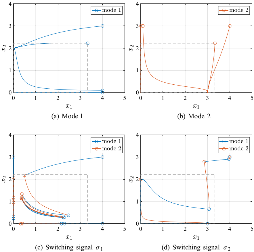
Fig. 2 Trajectories of the switched system in Example 1, for (a) individual mode 1 with initial states (4, 3), (4, 0.1), (4, 0), and (10/3, 20/9); (b) individual mode 2 with initial states (4, 3), (0.1, 3), (0, 3), and (10/3, 20/9); (c) switching signal \sigma_1 with initial states (4, 3), (4, 0), and (0, 3); (d) switching signal \sigma_2 with initial state (4, 3). The circles mark the beginning of a segment after switching. The dashed rectangles represent S = [0, 10/3] \times [0, 20/9]
