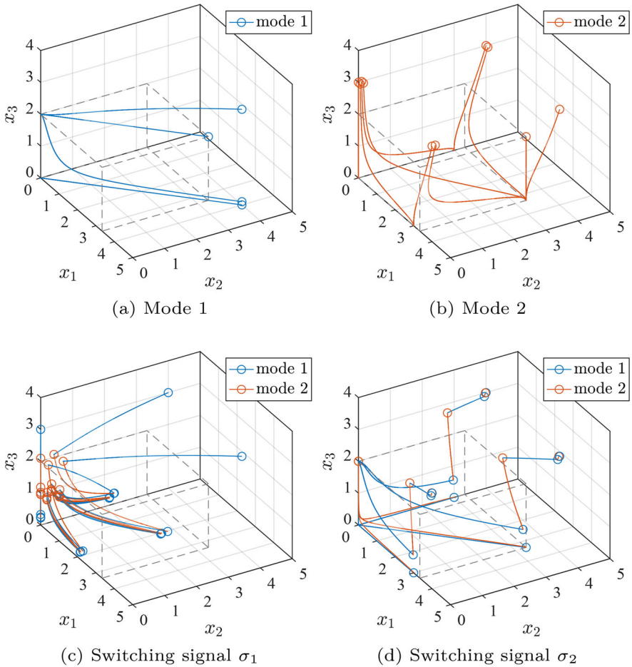
Fig. 3 Trajectories of the switched block-diagonal system in Example 2, for (a) individual mode 1 with initial states (4, 4, 3), (4, 4, 0.1), (4, 4, 0), and (10/3, 10/3, 2); (b) individual mode 2 with initial states (4, 4, 3), (4, 0.1, 3), (0.1, 4, 3), (4, 0, 3), (0, 4, 3), (0.1, 0.1, 3), (0.1, 0, 3), (0, 0.1, 3), (0, 0, 3), and (10/3, 10/3, 2); (c) switching signal \sigma_1 with initial states (4, 4, 3), (4, 0, 3), (0, 4, 3), and (0, 0, 3); (d) switching signal \sigma_2 with initial states (4, 4, 3), (4, 0, 3), and (0, 4, 3). The circles mark the beginning of a segment after switching. The dashed hyperrectangles represent S = [0, 10/3]^2 \times [0, 2]
