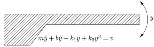
Fig. 1. MEMS device in Example 8.1. The following parameter values are consistent with the folded spring device in Zhang et al. (2002): m = 277 , b = 0.678 , k_1 = 7.61 , and k_3 = .0441 (in units of \mu Newtons, \mu meters, \mu seconds, and Volts).
