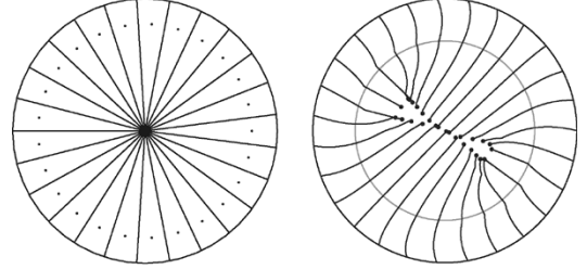
Fig. 3. Radial/spherical quantizer. (a) Quantization regions and points. (b) Closed-loop trajectories.
