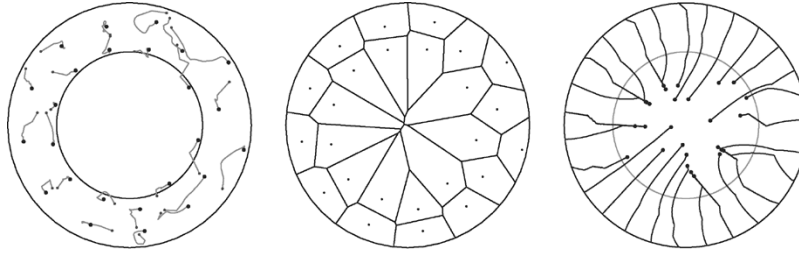
Fig. 4. Radially weighted quantizer. (a) Lloyd iterations. (b) Quantization regions and points. (c) Closed-loop trajectories.
