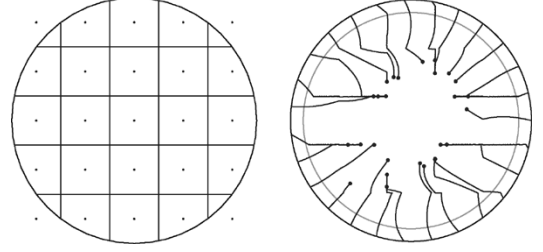
Fig. 1. Rectangular quantizer. (a) Quantization regions and points. (b) Closed-loop trajectories.
