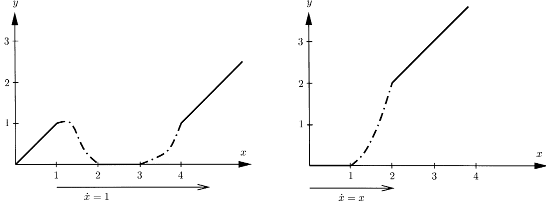
Fig. 1. Two counterexamples.
