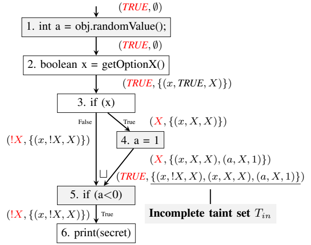
Fig. 3. An example shows an incomplete taint set. Assume getOptionX() is a constrain-API whose return value is represented by the symbolic value X .
