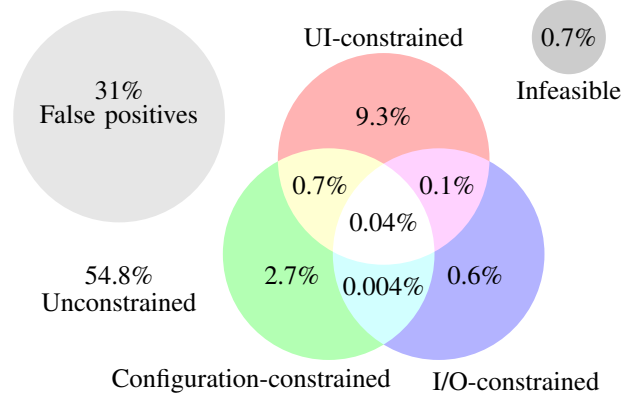
Fig. 4. Different types of taint flows.
