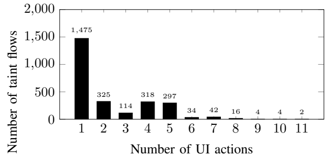
Fig. 5. The distribution of UI-constrained taint flows.
