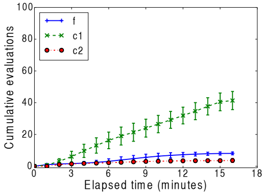
(c) Decoupled, \gamma = \infty
