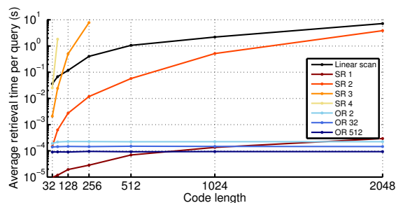
Figure 3. Empirical timing tests for different retrieval algorithms. SR: semantic retrieval, OR: ordered retrieval. The numbers next to “SR” and “OR” in the figure legend correspond to the semantic hashing radius and the terminal ordered retrieval neighborhood cardinality, respectively. As the code length increases, Hamming balls of very small radii become prohibitive to scan. Ordered retrieval carries a small fixed cost that is independent of code length.
