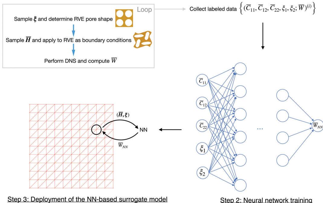
Fig. 4 The data-driven computational homogenization procedure consists of three steps: (1) building the offline training database by performing RVE calculations at the cellular level; (2) training the neural network to obtain a surrogate model for effective strain energy density; and (3) deploying the NN-based surrogate model for macroscopic problems.
