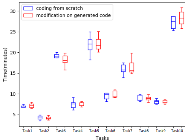
Fig. 6. Usefulness of Generated Programs (Group A)
