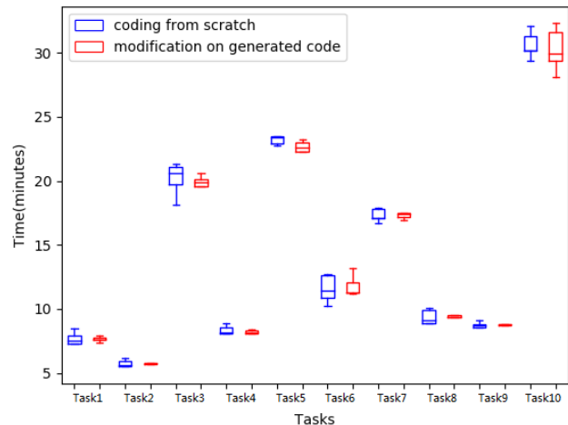
Fig. 7. Usefulness of Generated Programs (Group B)
