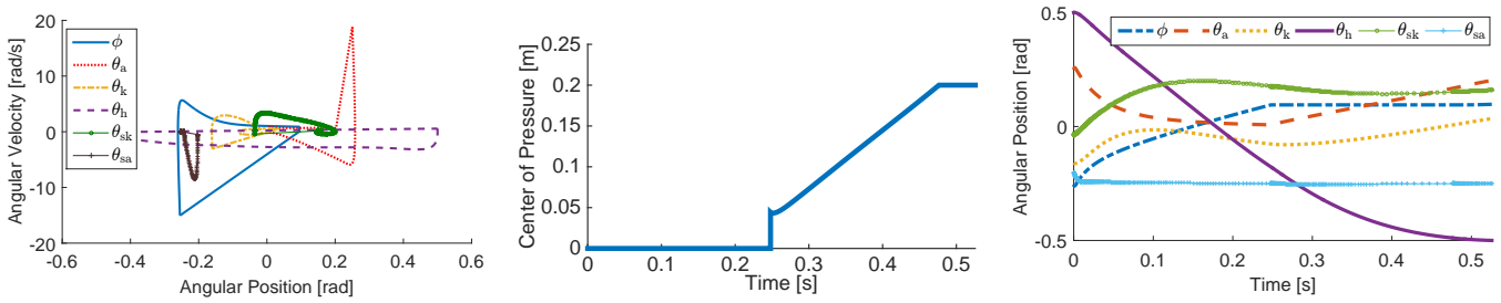
Fig. 5. Phase portrait (left), center of pressure (center), and angular positions (right) over one steady-state step of the nominal “human” gait.
