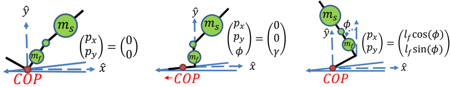
Fig. 2. Heel contact configuration (left), flat foot configuration (center), and toe contact configuration (right) during stance on a slope with angle \gamma .
