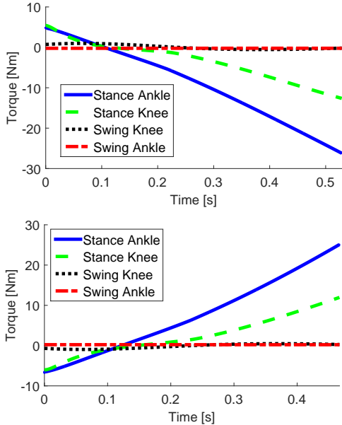
Fig. 6. The virtual BWS control torque with 24.5% BWS (top) and -24.5\% BWS (bottom) over one steady-state step.
