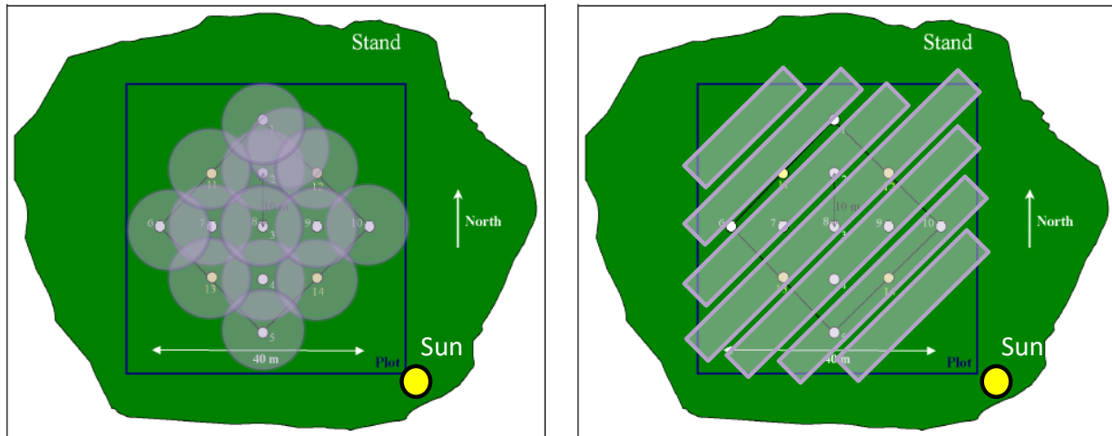
Figure 1: Spatial footprints of LAI-2000 (left) and TRAC (right) measurements following the CCRS sampling scheme (adapted from (Leblanc 2005c, Leblanc 2008)) for overstory LAI for a 40mx40m ESU. LAI-2000 footprints determined by canopy height while TRAC footprints are determined both by canopy height and solar zenith angle. Only every second TRAC footprint shown for clarity.
