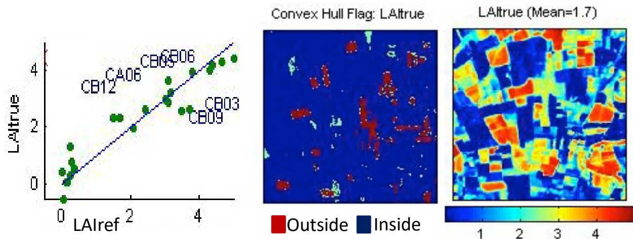
Figure 6: Outputs of VALERI reference LAI mapping process. Left panel shows scatter plot of predicted versus actual LAI based on robust linear regression. Outliers are indicated as alphanumeric symbols. Centre panel shows mask of areas within (blue) and outside (red)
