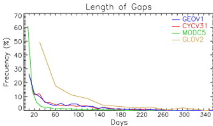
Figure 19: Gap length frequency for four Global LAI products over all BELMANIP2 sites for 3 years (Camacho et al. 2012).
