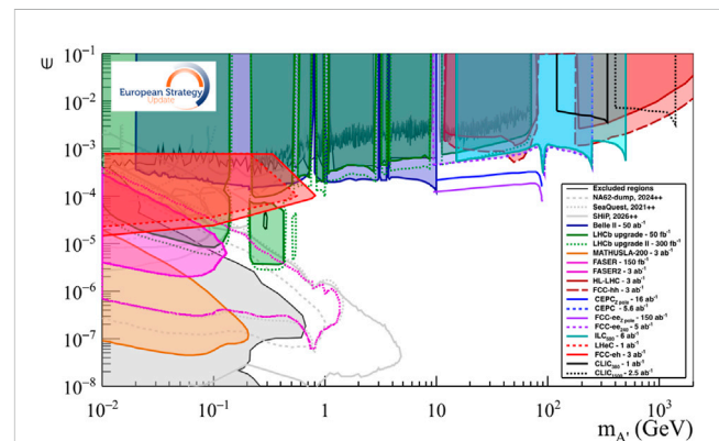
FIGURE 8 Exclusion reach for dark photons at various experiments as a function of the dark photon mass m_A and the mixing parameter between the dark and SM photon, \epsilon . Exclusion limits are computed at 95% CL in the case of FCC-ee, FCC-hh, and CepC, while the contour for the FC-eh corresponds to the observation of 10 signal events. All other limits are computed at 90% CL [31].
