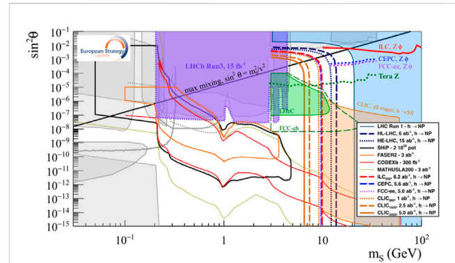
FIGURE 9 Exclusion reach in the m_S - \sin^2 \theta plane at various experiments. The symbols S and \phi are used interchangeably to identify the singlet. Exclusion limits are computed at 95% CL in the case of FCC-ee, FCC-hh, ILC, CLIC, and CepC, while all other limits are computed at 90% CL [31].
