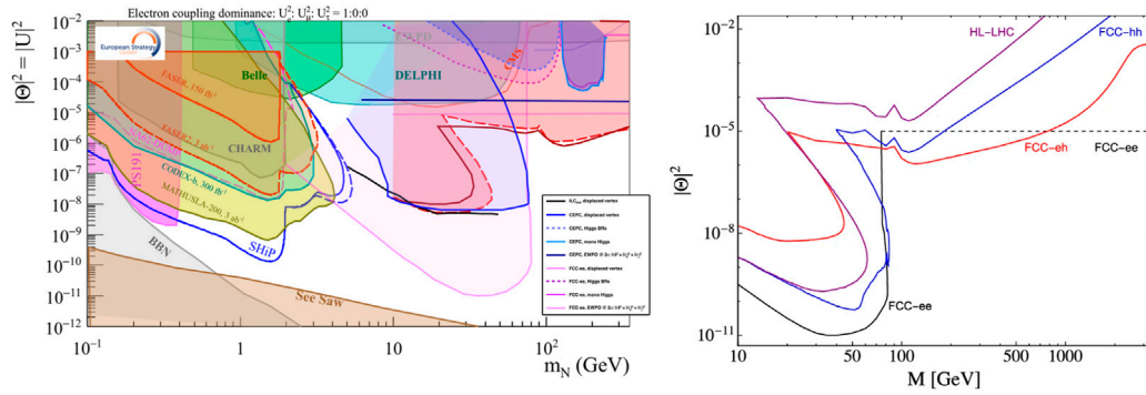
FIGURE 11 Left: Exclusion reach for minimal heavy lepton portal models assuming electron-coupling dominance in the |\Theta|^2 - m_N plane at various experiments. Exclusion limits are computed at 90% CL [31]. Right: Comparison of exclusion reaches at 90% CL from searches at the HL-LHC, FCC-hh, and FCC-eh and precision measurements at the FCC-ee [57].
