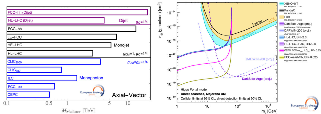
FIGURE 7 Left: Exclusion reach at 95% CL for axial-vector simplified models at future colliders assuming a DM mass of M_{DM} = 1 GeV. Right: Results from searches for invisible decays of the Higgs boson, assuming a Majorana-type DM, compared to constraints of current and future direct detection experiments on the spin-independent WIMP–nucleon scattering cross section [31]. The region where the irreducible background from neutrinos may hide a DM signal, usually labeled as the “neutrino floor,” is not reported. For further reading, a recent paper on the subject is given in Ref. [50].
