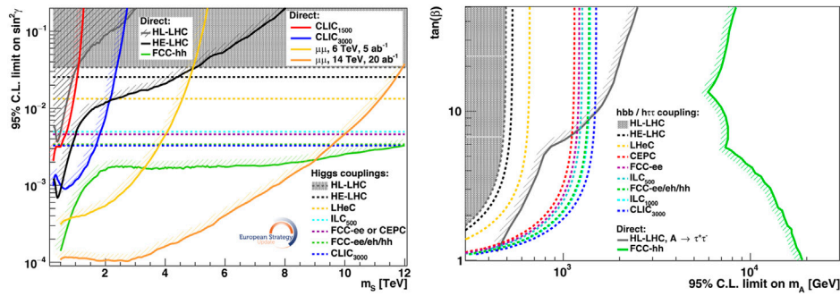
FIGURE 3 Exclusion reach obtained from the precision measurements of the Higgs boson couplings and from direct searches for new states. Left: Sensitivity in the plane \sin^2\gamma - m_S , where \gamma and m_S are the mixing angle and the mass of the singlet mixing with the SM Higgs boson, respectively. Right: Sensitivity in the plane \tan\beta - m_A , where \tan\beta is the ratio of the vacuum expectation value for the two Higgs doublets and m_A is the mass of the CP-odd scalar Higgs boson, in a type-II two-Higgs doublet model [31].
