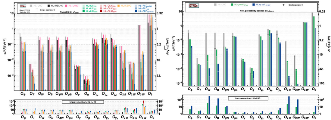
FIGURE 12 Probability reach for the Wilson coefficients computed at 68% CL from the global fit (solid bars). The vertical “T”-shaped lines report the results obtained if only one operator is generated by the UV dynamics. Left: Reach of all options considered in Ref. [38]. Right: Sensitivity of the muon collider at both \sqrt{s} = 3 and 10 TeV, compared to that of the HL-LHC [30].
