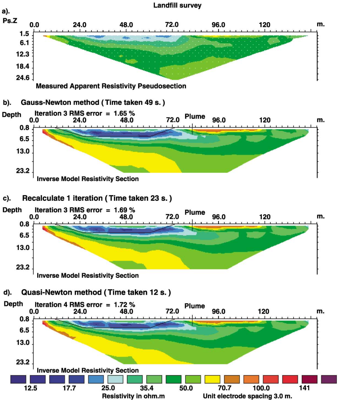
Fig. 6. (a) Apparent resistivity pseudosection from the landfill survey. Inversion models obtained with the (b) Gauss–Newton method, (c) recalculation of the Jacobian matrix for one iteration and (d) quasi-Newton method. The outline of the landfill is superimposed on the inversion models.
