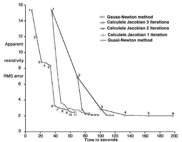
Fig. 3. Change of apparent resistivity RMS error with computer CPU time for the different methods in the inversion of the rectangular prism model data set. The iteration numbers for the Gauss–Newton and quasi-Newton methods are also shown.
