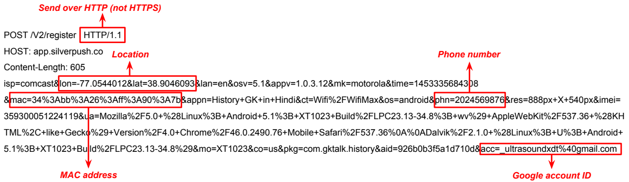
Fig. 1. An example of an insecure, non-standardized implementation of the ultrasound-enabled applications. HTTP POST request sent by an ultrasound-enabled app that we found on the Google Play Store, violating the user’s privacy and security practices: (1) The framework surreptitiously collects the user’s private information, including the Google account ID, phone number, geolocation, the device MAC address, and other information; (2) The data is sent insecurely over HTTP (instead of HTTPS).
