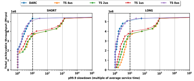
Figure 10. Simulating single queue preemptive systems with various overheads. At the microsecond scale, implementing and orchestrating preemptive systems remains challenging.
