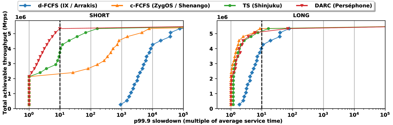
Figure 1. Simulated achievable throughput as a function of 99.9th percentile slowdown for the policies listed in Table 1 on a 16 cores system and a workload composed of 99.5% short requests ( 0.5\mu\text{s} ) and 0.5% long requests ( 500\mu\text{s} ). For a target SLO of 10 times the average service time for each request type, c-FCFS and TS can only handle 2.1 and 3.7 Millions requests per second (Mrps), respectively. DARC can sustain 5.1 Mrps for the same objective. The Y axis represents the total achievable throughput for the entire workload.
