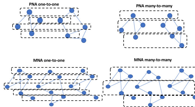
Figure 1. The figure shows an example of PNA one-to-one, PNA many-to-many, MNA one-to-one, and MNA many-to-many.
