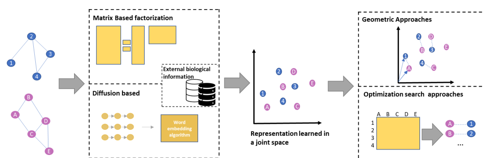
Figure 2. The figure shows the proposed taxonomy of the considered NE-NA algorithms for PPI networks based on their general pipeline.
