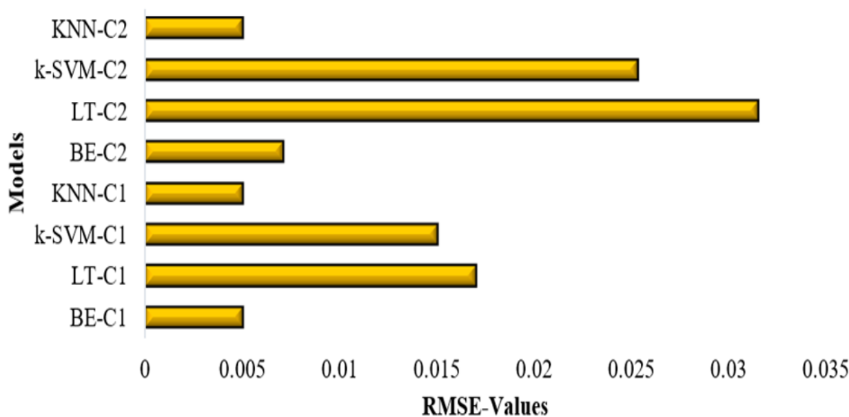
Figure 10. Performance of the model prediction of floods using the RMSE values.
