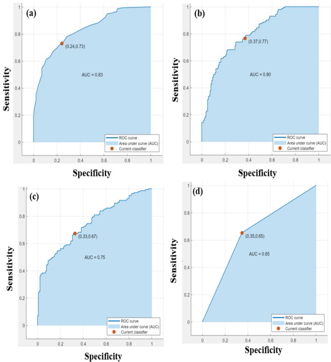
Figure 9. Performance of the model for the spatial prediction of flash floods using the ROC curve technique and AU for (a) EB-C2, (b) LT-C2, (c) k-SVM, (d) KNN-C2 algorithms.
