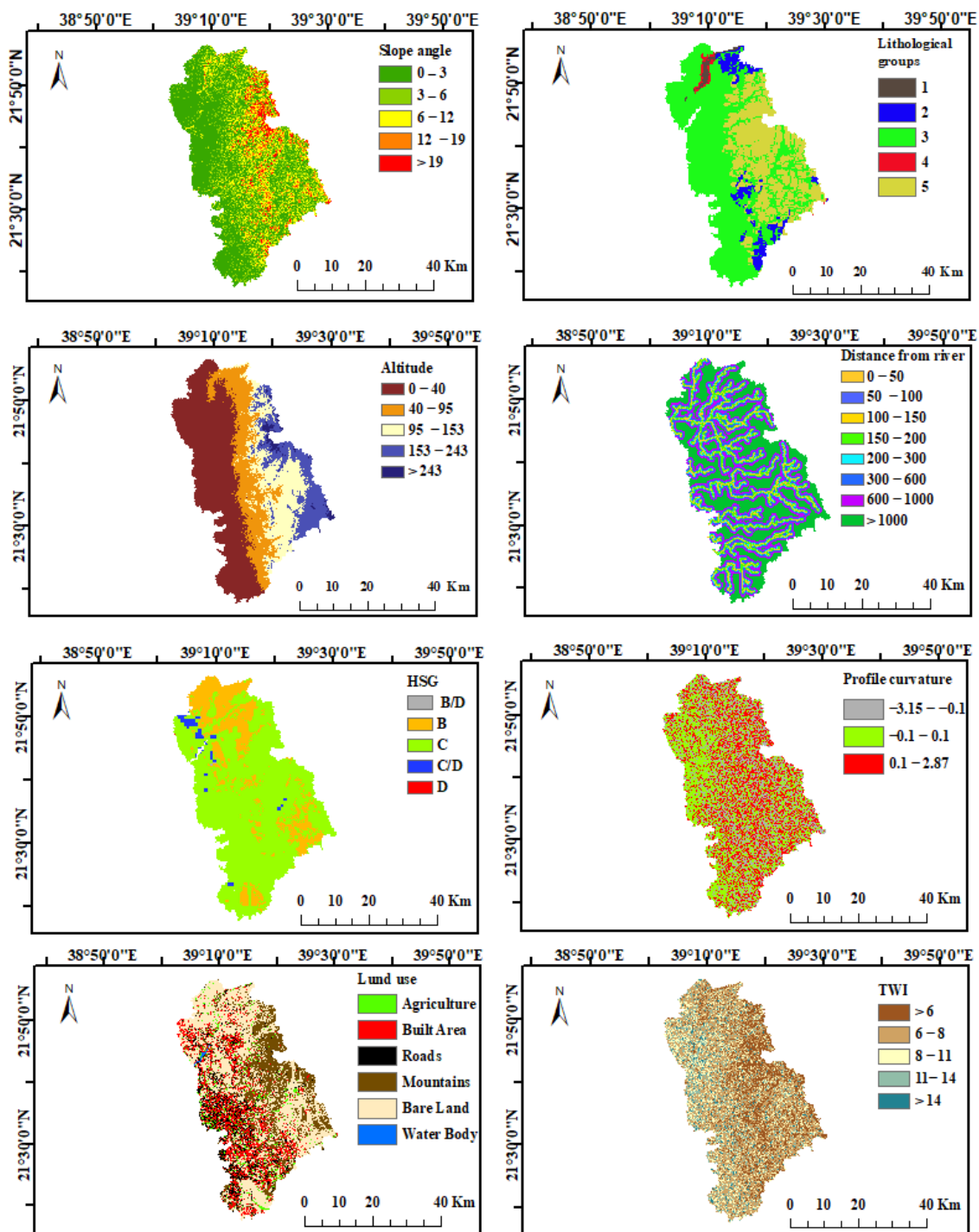
Figure 2. Flood condition factors based on the study area.
