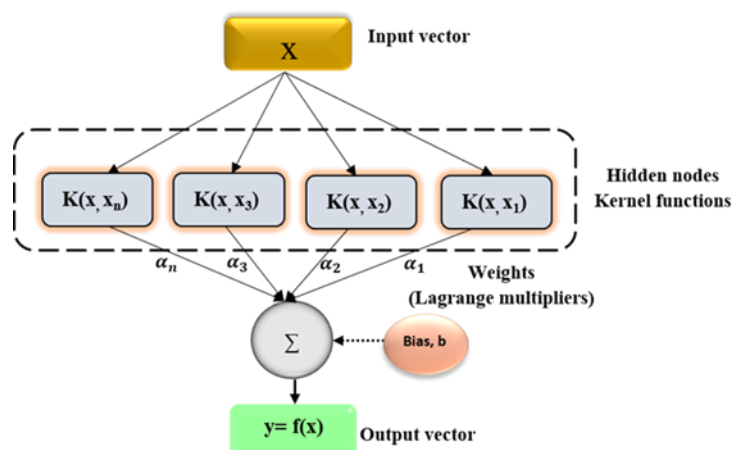
Figure 5. Structure of the k-SVM model.
