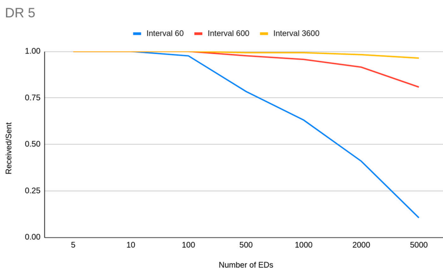
Figure 7. DR5 capacity related to transmission interval.
