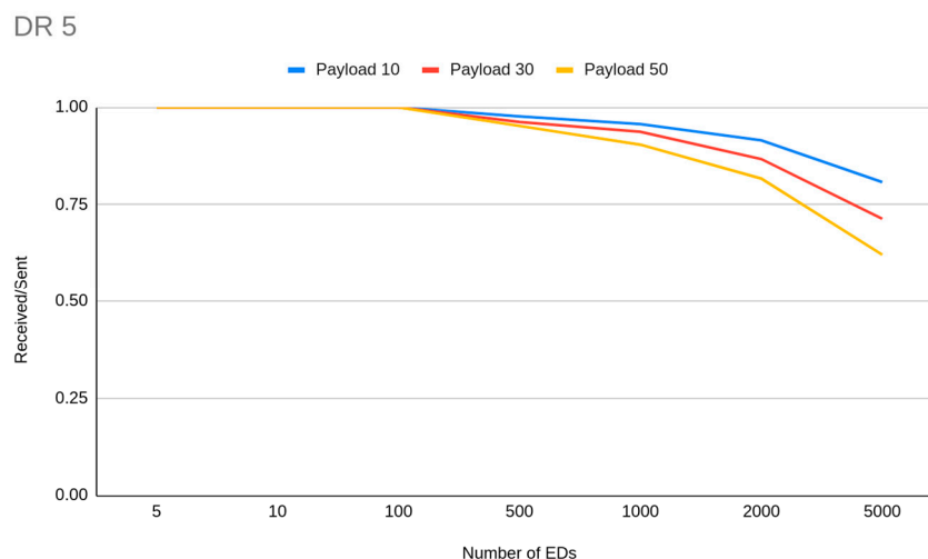
Figure 8. PDR differentiation derived from payload size and transmission interval relation.
