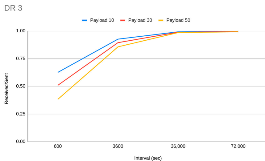
Figure 6. PDR differentiation derived from payload size and transmission interval relation.
