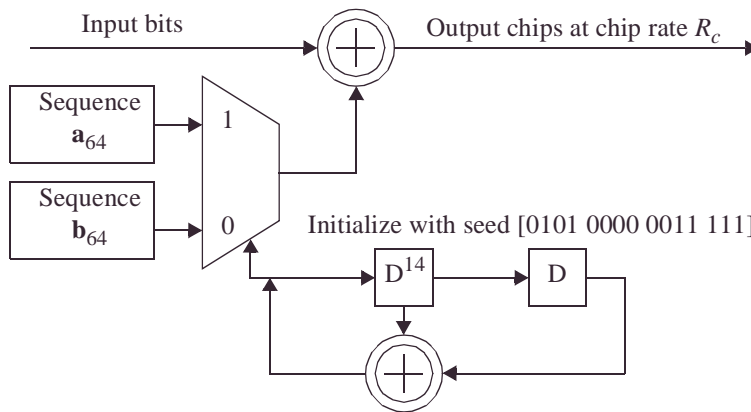
Figure 27—Realization of the CMS code spreading
