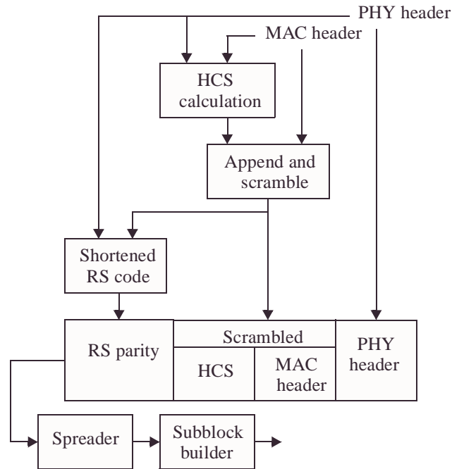
Figure 29— Frame header construction process for CMS
