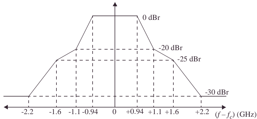
Figure 2—Transmit spectral mask
