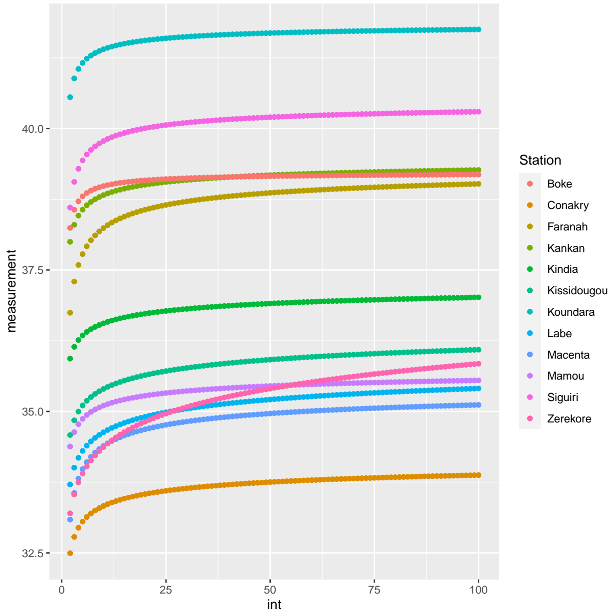
Figure S4. Estimates of \chi_T versus T = 2, 3, \dots, 100 for all twelve stations.
