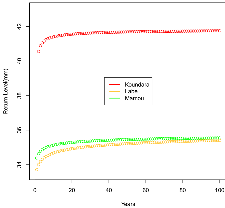
Figure S2. Estimates of x_T versus T = 2, 3, \dots, 100 for middle Guinea.
