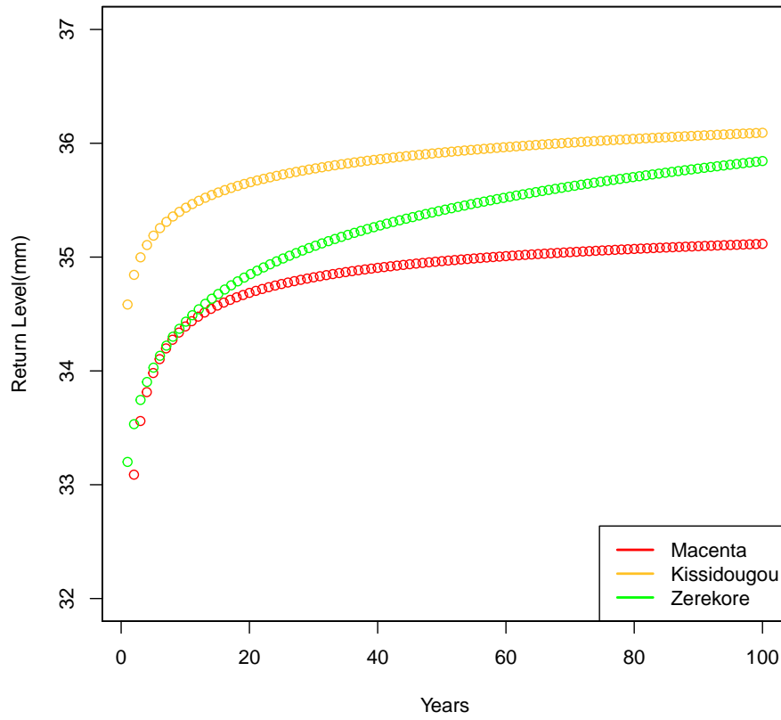
Figure S1. Estimates of x_T versus T = 2, 3, \dots, 100 for forested Guinea.
