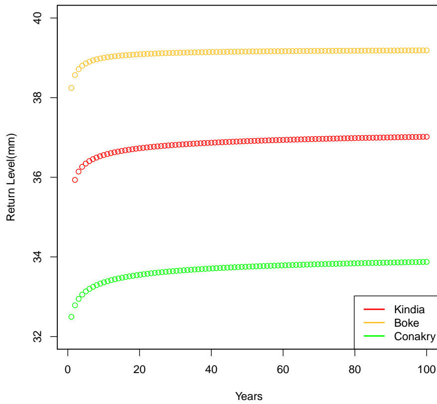
Figure S3. Estimates of x_T versus T = 2, 3, \dots, 100 for coastal/maritime Guinea.
