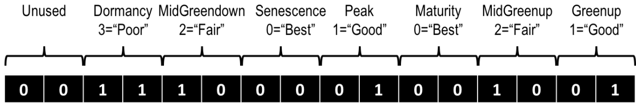
Figure 2: An example QA_Detailed 16-bit integer value, its binary representation, and associated phenometric-specific bit pair interpretation.
