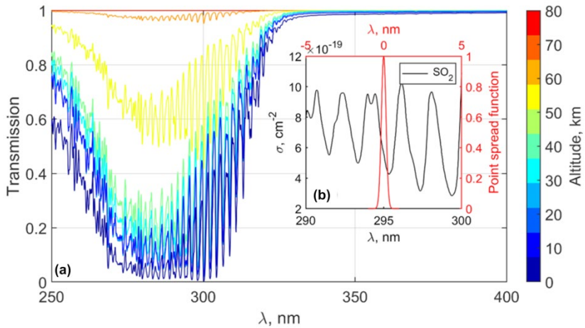
Fig. 2. Examples of \text{SO}_2 transmission spectra, modeled for DAVUS measurements at different atmospheric altitudes (a). All spectra are convolved by a point spread function of the instrument with a spectral width of 0.2 nm (b)
