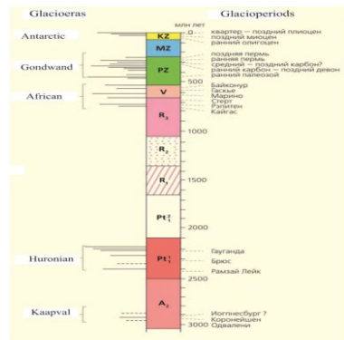
Fig. 4. Glacioeras and glacioperiods in interval from Late Archean to the present [10]. Long period of glacioceros absence between Huronian and African glacioceros is “Great Ice Pause”
