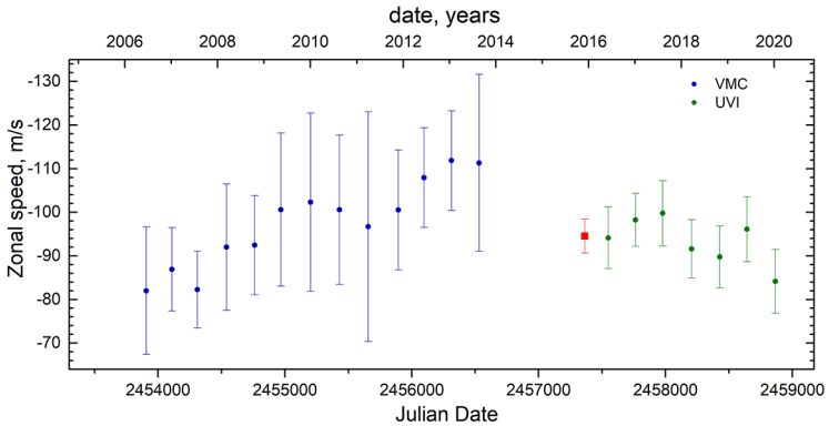
Fig. 1. Variations of the mean zonal wind speed at 20^\circ \pm 2.5^\circ \text{S} over the mission time (X axis – Julian Date) from 11:00 to 13:00 LT. Every point is the result of averaging over the Venusian year (224.7 days) in latitude band 20^\circ \pm 2.5^\circ \text{S} . Blue circles show zonal wind averaged through the Venusian year derived from VMC images, green circles are the same for UVI. Red square shows zonal wind averaged by using only two days of observation (2015.12.07–08). Error bars correspond to standard deviation \sigma .
