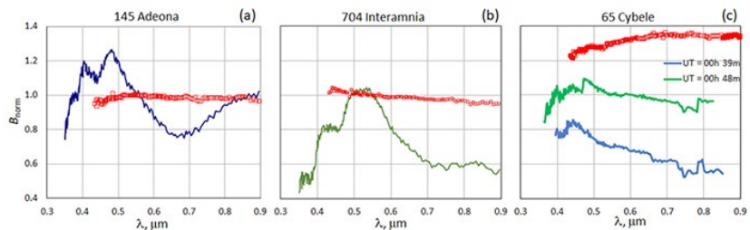
Fig. 1. The reflectance spectra (normalized at 0.55 \mu\text{m} ) B_{norm} measured in AAs 145, 704 (in September 2012), and 65 (in September 2016). The classical SMASSII spectra [5] of these asteroids are shown by red symbols. In panel (c) the spectra are shifted in vertical relative each other
