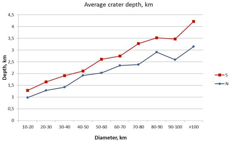
Fig. 2. Distribution of average crater depth of the northern and southern polar regions in dependence of craters diameters.
