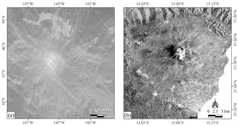
Fig. 1: a) Idunn Mons ( 46^{\circ} S; 146^{\circ} W), Imdr Regio – Venus. Magellan left-look SAR scene - Resolution \sim 75 m, b) Mt. Etna ( 37.75^{\circ} N, 14.99^{\circ} E), Sicily – Italy. S-1 GRDH SAR Ascending – Resolution \sim 75 m
