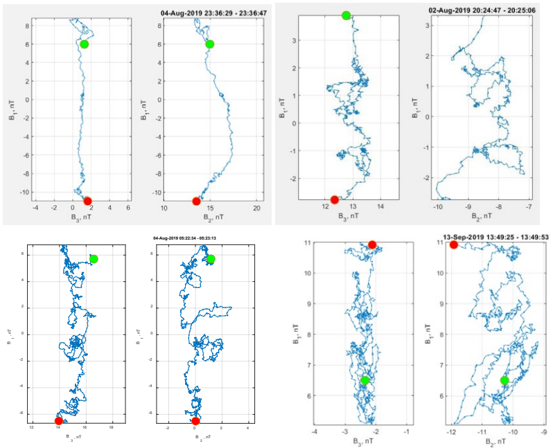
Fig. 2. 4 cases of magnetic structures within magnetopause of Mars at ~60° SZA. Different crossings of magnetopause show M and N components of the magnetic field
