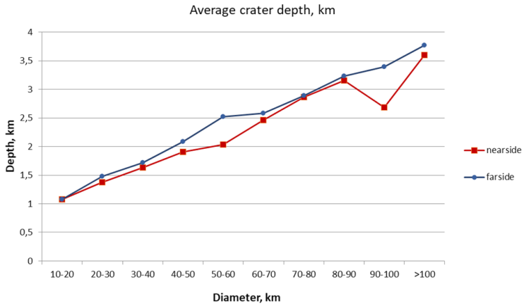
Fig. 3. Distribution of average craters depth on the near and far sides of the polar regions. The similar character is observed on both graphics.
