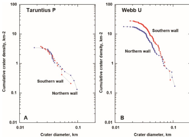
Fig. 2. Crater cumulative densities on the northern and southern walls. A: Identical densities of the younger, 1.55 Ga, crater Taruntius P. B: Cumulative crater density on the southern (poleward) wall of ancient, 3.11 Ga, crater Webb U is significantly higher for the superposed craters larger than \sim 60 m.
