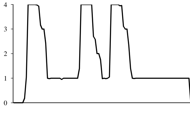
Figure 6. Build parallelism.
