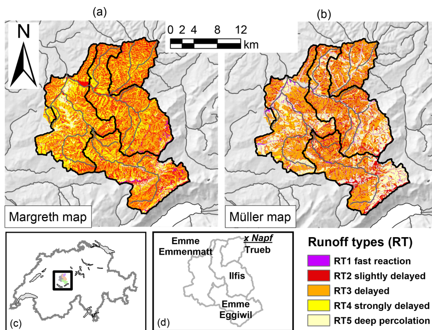
Figure 1. Overview on the investigated Emme catchment. (a) a process map according to Margreth et al. (2010); (b) a process map according to Müller et al. (2009); (c) the location of the target area within Switzerland and (d) the situation of the nested sub-areas and location of the Napf meteorological station. GIS elements are reproduced by kind authorisation of swisstopo (JA022265), BFS GEOSTAT/BUWAL.
