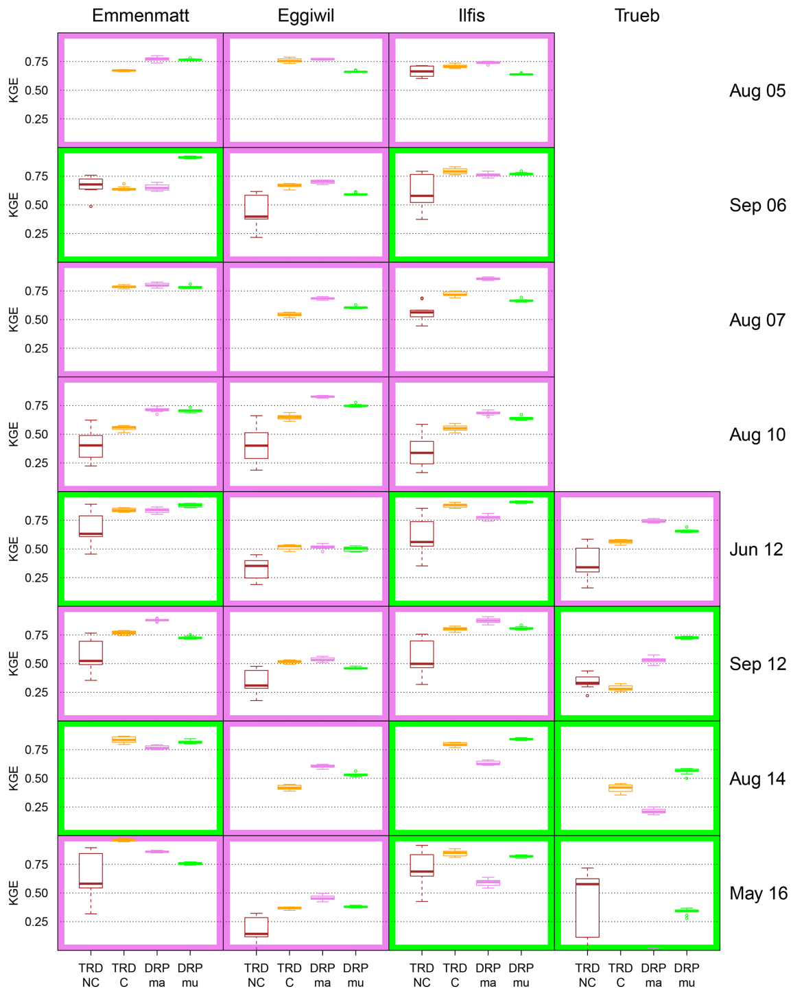
Figure 4. Re-analysis of eight large runoff events from 2005 to 2016 with CombiPrecip data in the four Emme catchments. The box plots represent the simulation results of the different model configurations. TRD-NC stands for uncalibrated PREVAH, TRD-C for calibrated PREVAH, DRP-ma for RGM-PRO relying on Margreth maps and DRP-mu for RGM-PRO based on Müller maps. The border colour reveals whether DRP-ma (pink) or DRP-mu (light green) performed better in terms of median KGE. Where no box plot is visible, all KGE values were below zero. The spread in KGE of uncalibrated PREVAH results from 10 random hydrological parameter sets out of 4000 Monte Carlo simulations, whereas uncertainty from calibrated PREVAH originates from the 10 parameter sets with highest KGE for the May 2016 event in Emmenmatt. The spread in RGM-PRO arises from simulations with 10 hydrological parameter sets lying in narrow ranges determined by sprinkler experiments (Antonetti et al., 2017).
