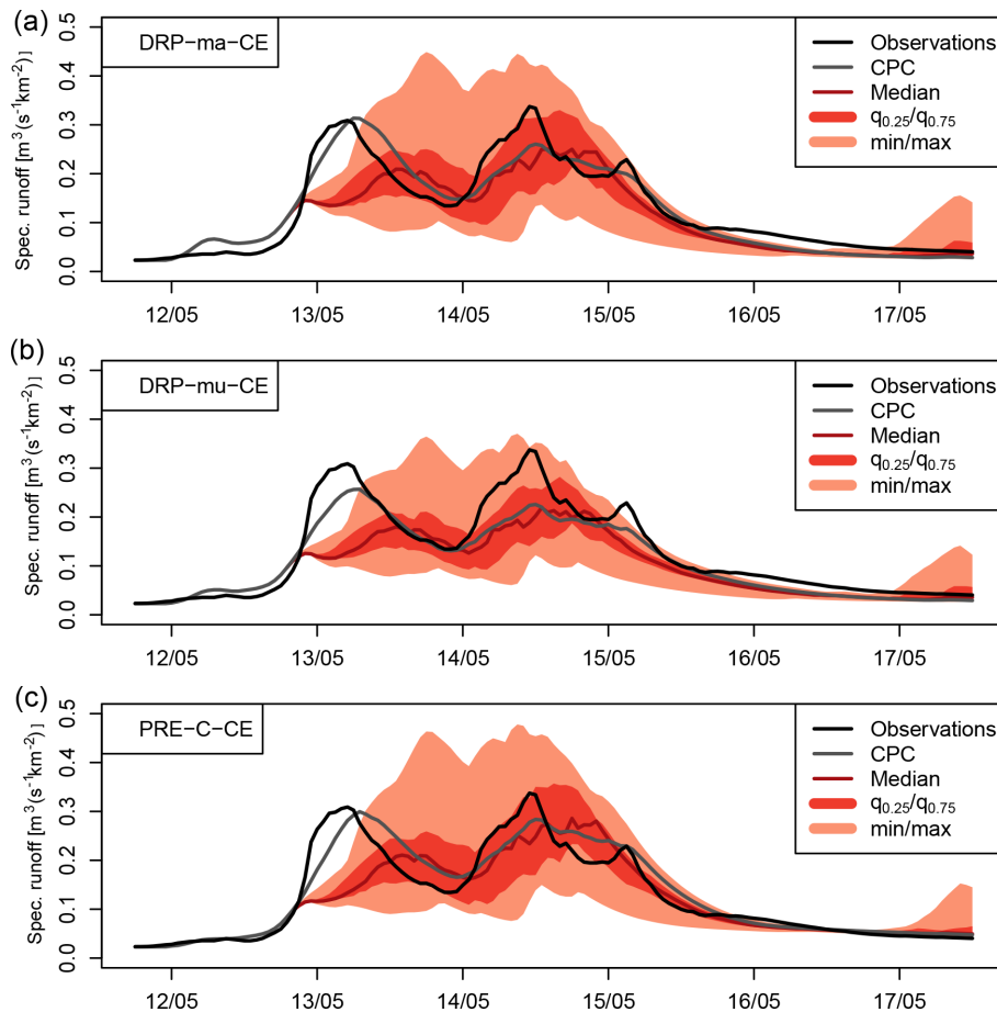
Figure 6. Probabilistic forecasts for the Emmenmatt catchment with a switch to the forecast mode on 12 May at 19:00 for (a) DRP-ma-CE, (b) DRP-mu-CE and (c) PRE-C-CE.
