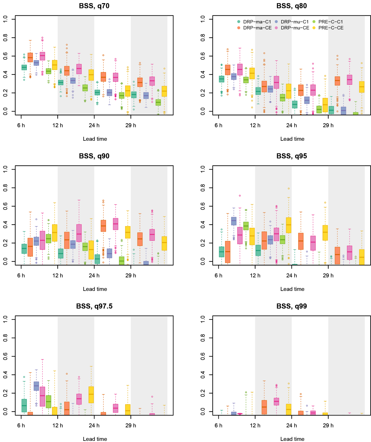
Figure 8. Comparison of BSS in the Emmenmatt catchment for deterministic DRP-ma-C1, DRP-mu-C1 and PRE-C-C1 and probabilistic DRP-ma-CE, DRP-mu-CE and PRE-C-CE as a function of lead time for several threshold quantiles for all events in the investigated period from May until July 2016. A window of 6 h was taken for the computations. The box plots represent the sampling uncertainties of the score computations obtained with bootstrapping.
