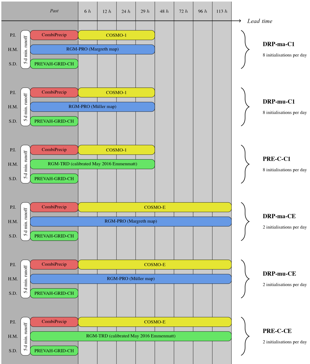
Figure 3. Scheme of the FF forecasting chains in the Emme catchments investigated in this paper, with the key indicated on the right-hand side. On the left-hand side, P.I. stands for precipitation input, H.M. for hydrological model and S.D. for soil moisture data. “5 d min. runoff” represents the minimum observed runoff in the last 5 days prior to the forecast.
