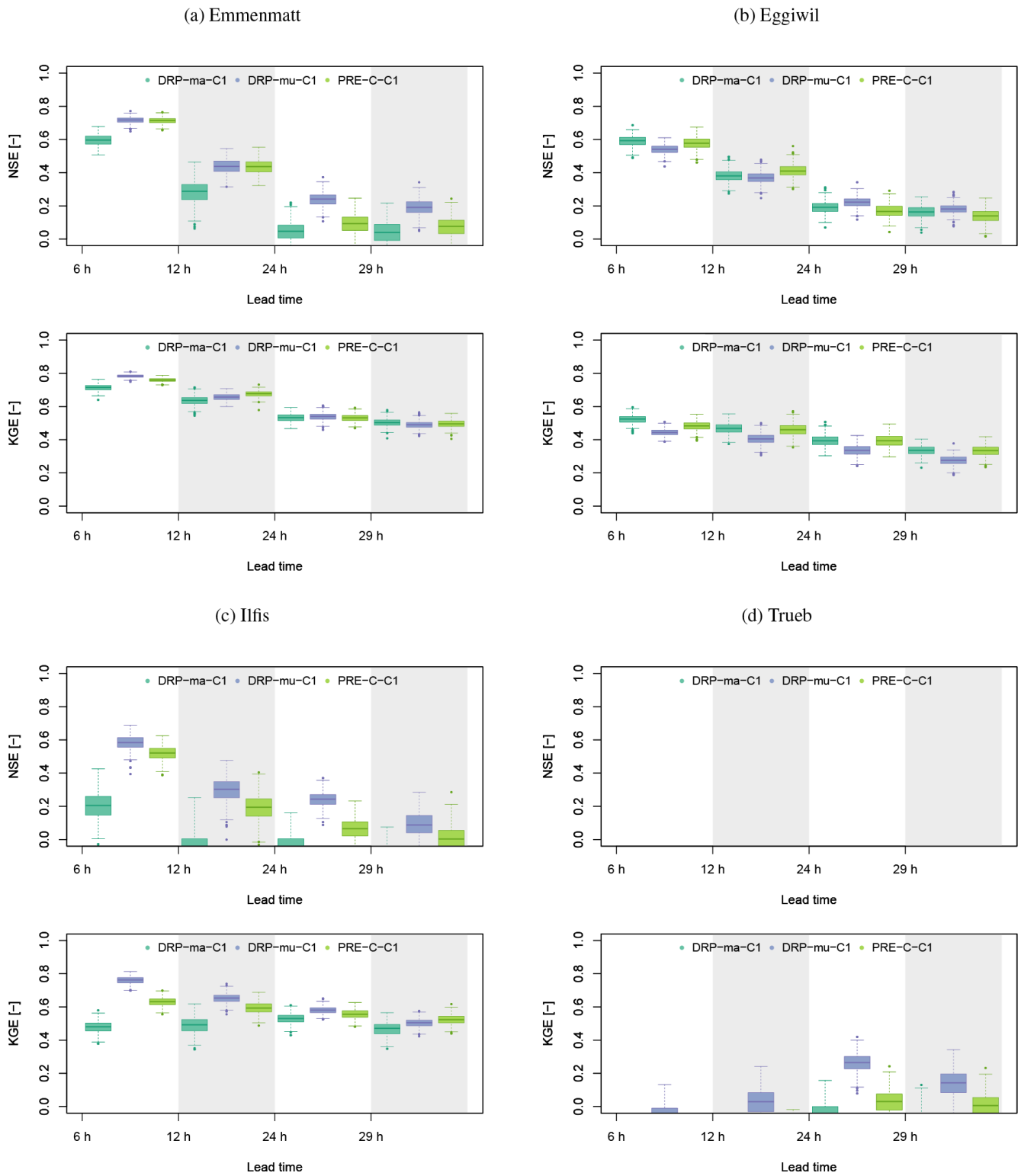
Figure 7. NSE and KGE for (a) Emmenmatt, (b) Eggiwil, (c) Ilfis and (d) Trueb as a function of lead time for DRP-ma-C1 (dark green), DRP-mu-C1 (blue) and PRE-C-C1 (light green) for all events in the investigated period from May until July 2016. A window of 6 h was taken for the computations, e.g. from 19 to 24 h for the 24 h lead time. The box plots represent the sampling uncertainties of the score computations obtained with bootstrapping (Addor et al., 2011).
