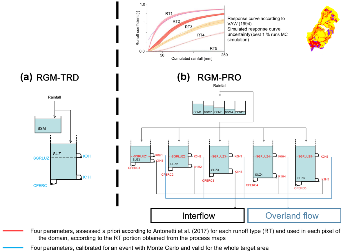
Figure 2. Structure of the adopted RGMs. (a) RGM-TRD module from the traditional PREVAH model, with four parameters requiring calibration (Gurtz et al., 2003) and validity for the whole target area. (b) RGM-PRO module using typical infiltration curves for a priori estimation of four parameters for five runoff types (Table 2) according to Antonetti et al. (2017) and Antonetti et al. (2016b). RTs are obtained from process maps (Fig. 1).
