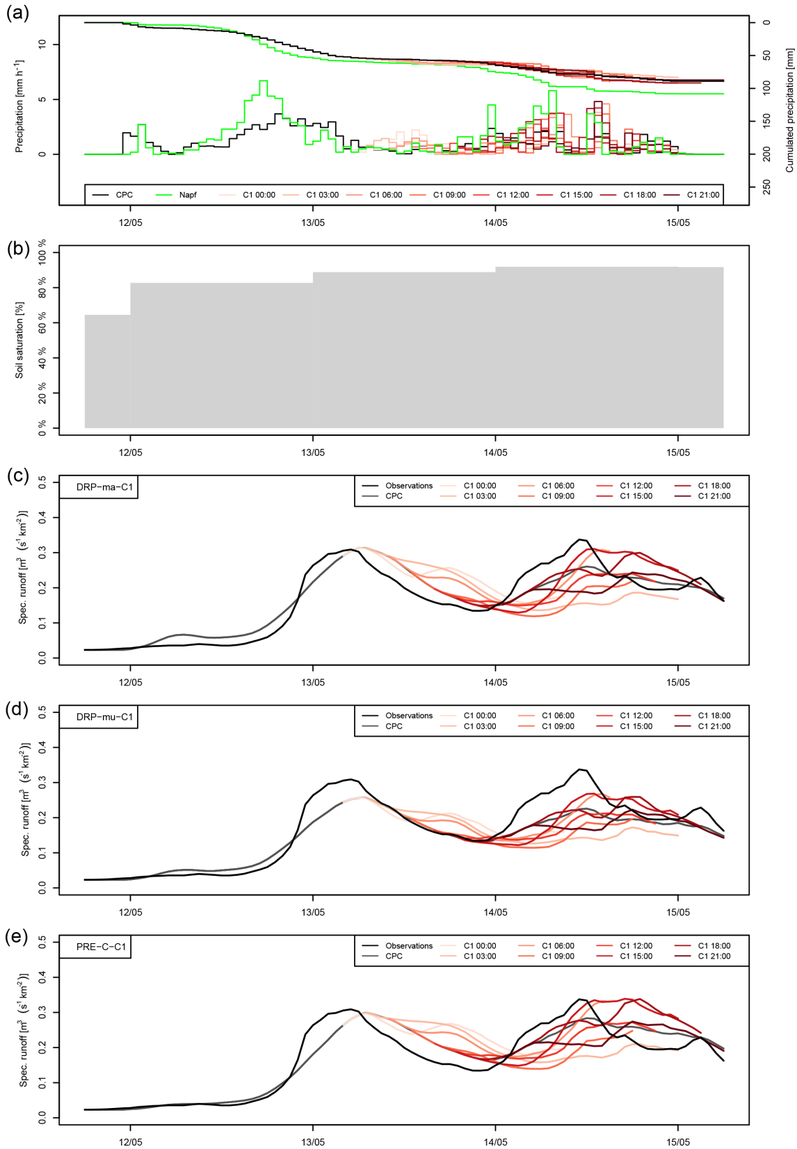
Figure 5. Flood predictions with (c) DRP-ma-C1, (d) DRP-mu-C1 and (e) PRE-C-C1 for Emmenmatt with eight initialisations each on the alert date of 13 May 2016. Catchment precipitation predictions from COSMO-1 and measurements from the Napf station and CombiPrecip (both provided by MeteoSwiss) are depicted in (a), and evolution of soil moisture from PREVAH simulations is depicted in (b).
